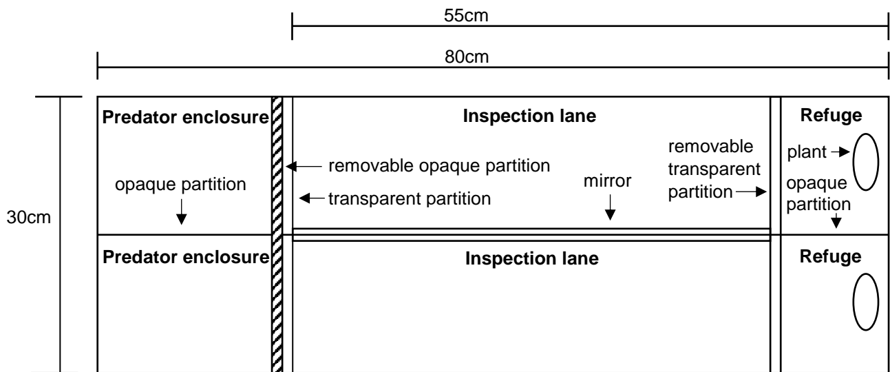
Schematic drawing of a predator inspection test tank. The tank is divided lengthwise into two identical, fully separated test arenas.
