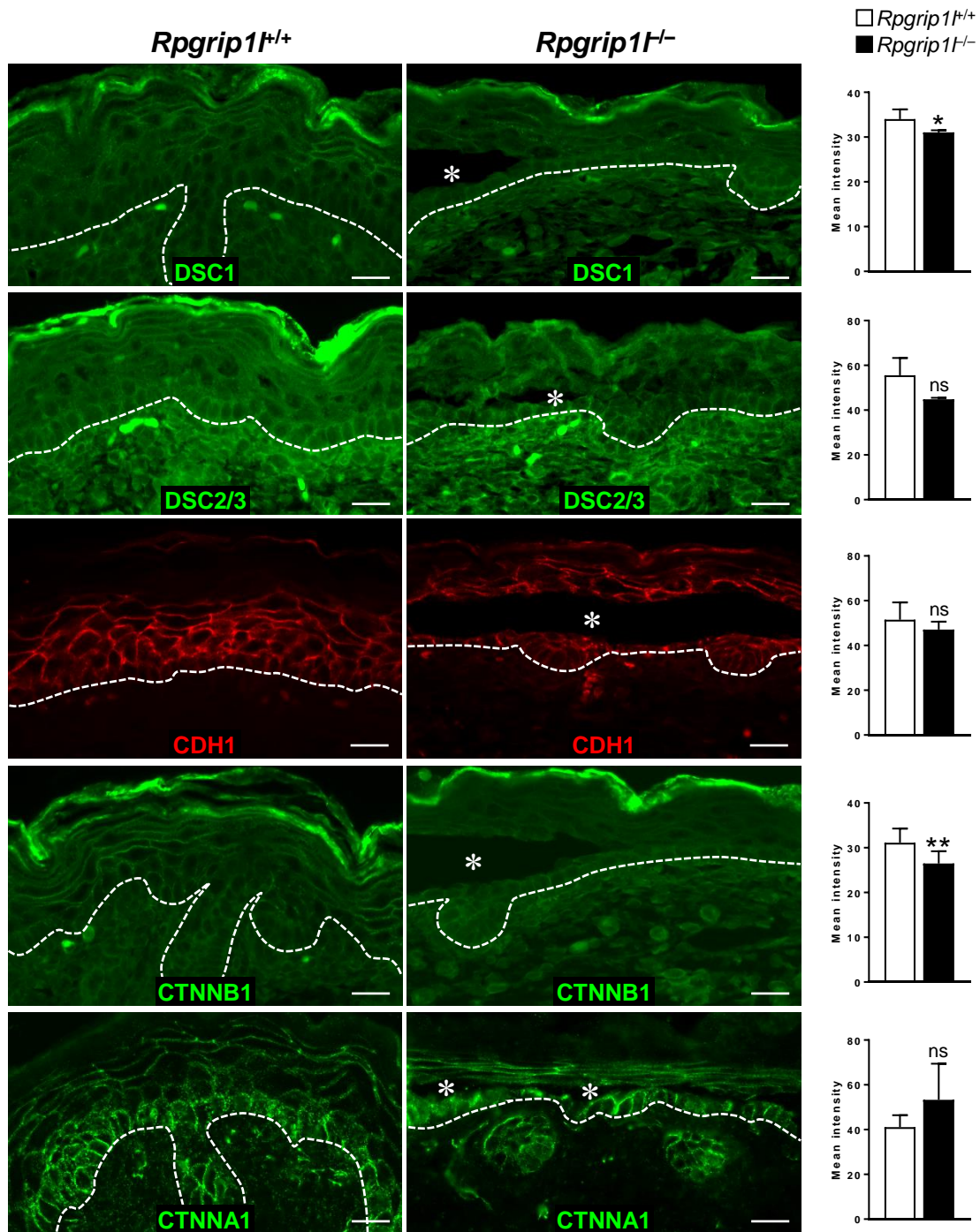
S3 Fig. Junctional proteins in E18.5 epidermis. Immunofluorescence labeling of desmocollins (DSC1, DSC2/3, green), E-cadherin (CDH1, red), \alpha -catenin (CTNNA1, green), and \beta -catenin (CTNNB1, green) in back skin of E18.5 control ( Rpgrip1 +/+ ) and homozygous ( Rpgrip1 -/- ) mutants. Dotted lines illustrate epidermal-dermal junction. Asterisks indicate intraepidermal blisters. Scale bar, 20 \mu m.
