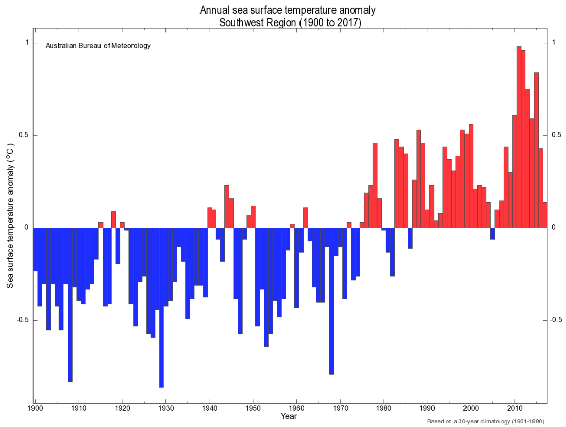
Figure S3: Annual sea surface temperature anomalies from 1900-2017. The 2011 and 2012 heatwave events produce the two highest peaks —Extracted from the Bureau of Meteorology time series graphs [9].
