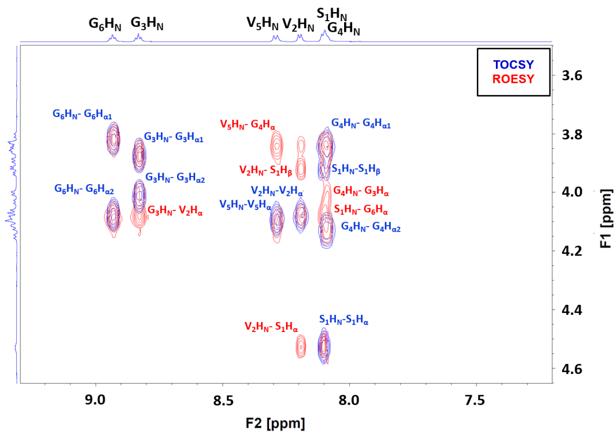
Figure S17. Fingerprint region of the 2D spectra for V1S at 288K, with TOCSY peaks shown in blue and ROESY peaks shown in red. 1D spectra correspond to the H N region (top) and the H α region (side). The peptide was dissolved in 90:10 H 2 O:D 2 O at a concentration of roughly 3.0 mM.
