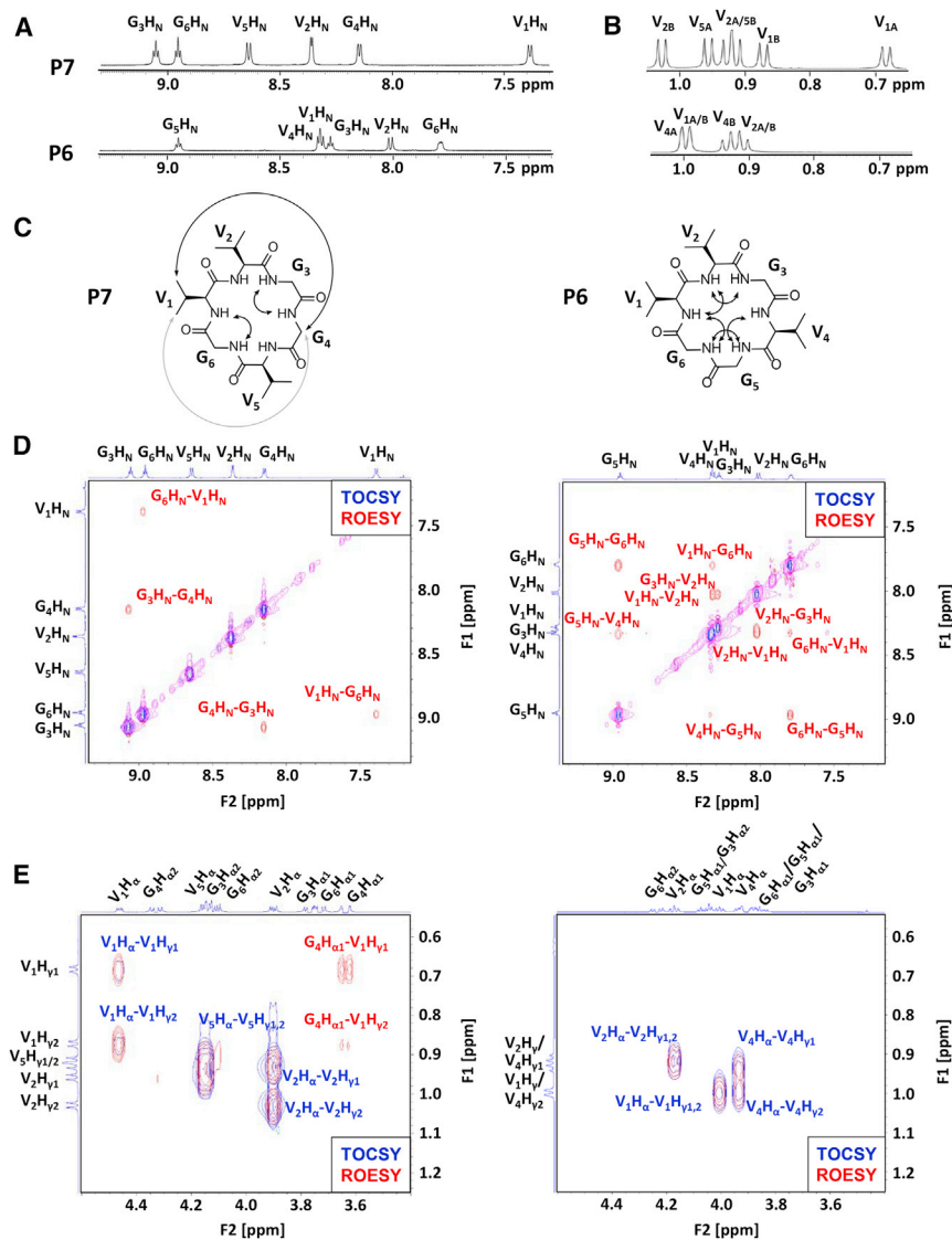
FIGURE 2 2D-NMR data for peptides P7 (cyclo-VVGGVG) and P6 (cyclo-VVGVGG) in water. (A) Amide proton region of ^1\text{H} NMR for P7 and P6. (B) Methyl proton region of ^1\text{H} NMR for P7 and P6. (C) Double-headed arrows show strong (black) and weak (gray) NOEs from the ROESY spectra for P7 and P6. (D) Amide-to-amide proton region of the TOCSY and ROESY spectra for P7 and P6. NOE crosspeaks are expected for positions at which \beta turns predominate in the solution ensemble. (E) \alpha -to-methyl proton region of the TOCSY and ROESY spectra for P7 and P6. NOE crosspeaks show medium-range interactions between methyl protons and \alpha protons. To see this figure in color, go online.
