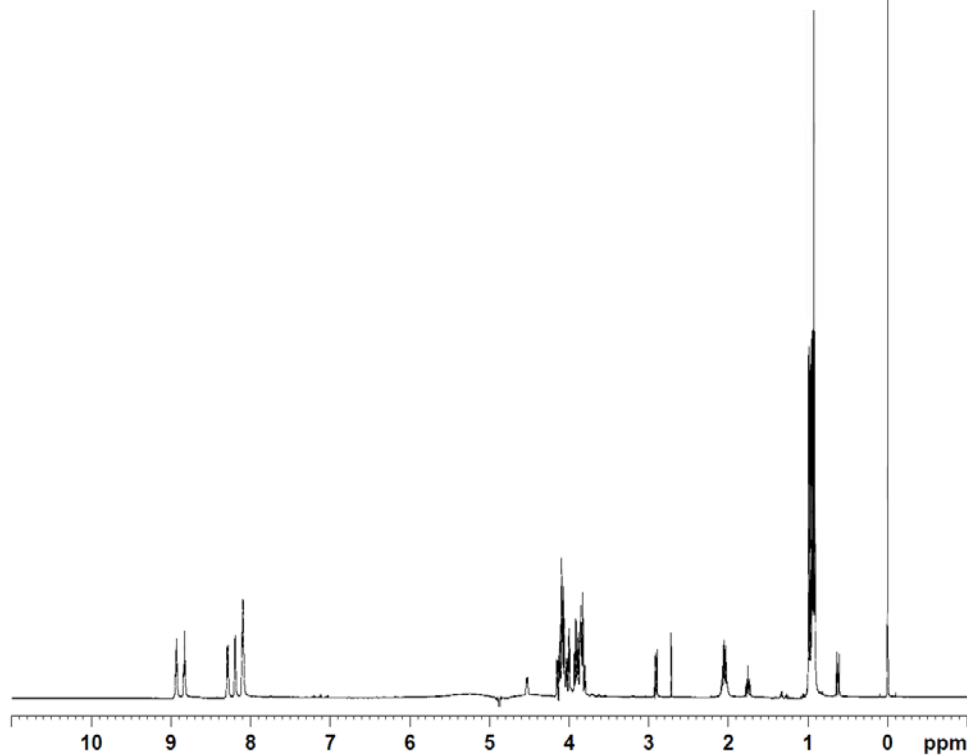
Figure S10. Complete 1 H NMR spectrum of VIS in 90:10 H 2 O:D 2 O at 288 K.
