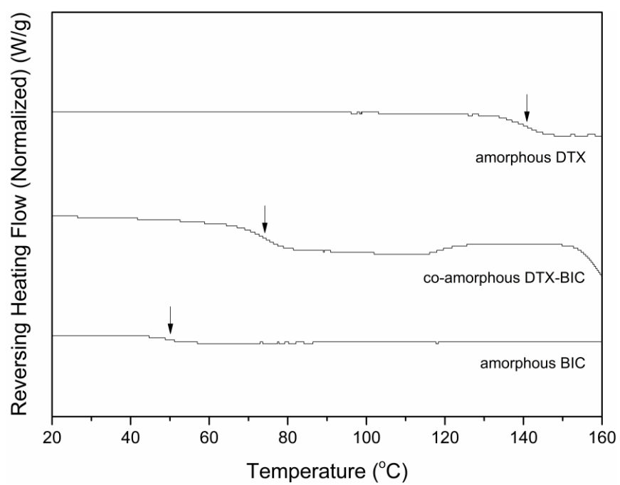
Figure S1: Thermograms of amorphous DTX, amorphous BIC and co-amorphous DTX-BIC after ball milling.
