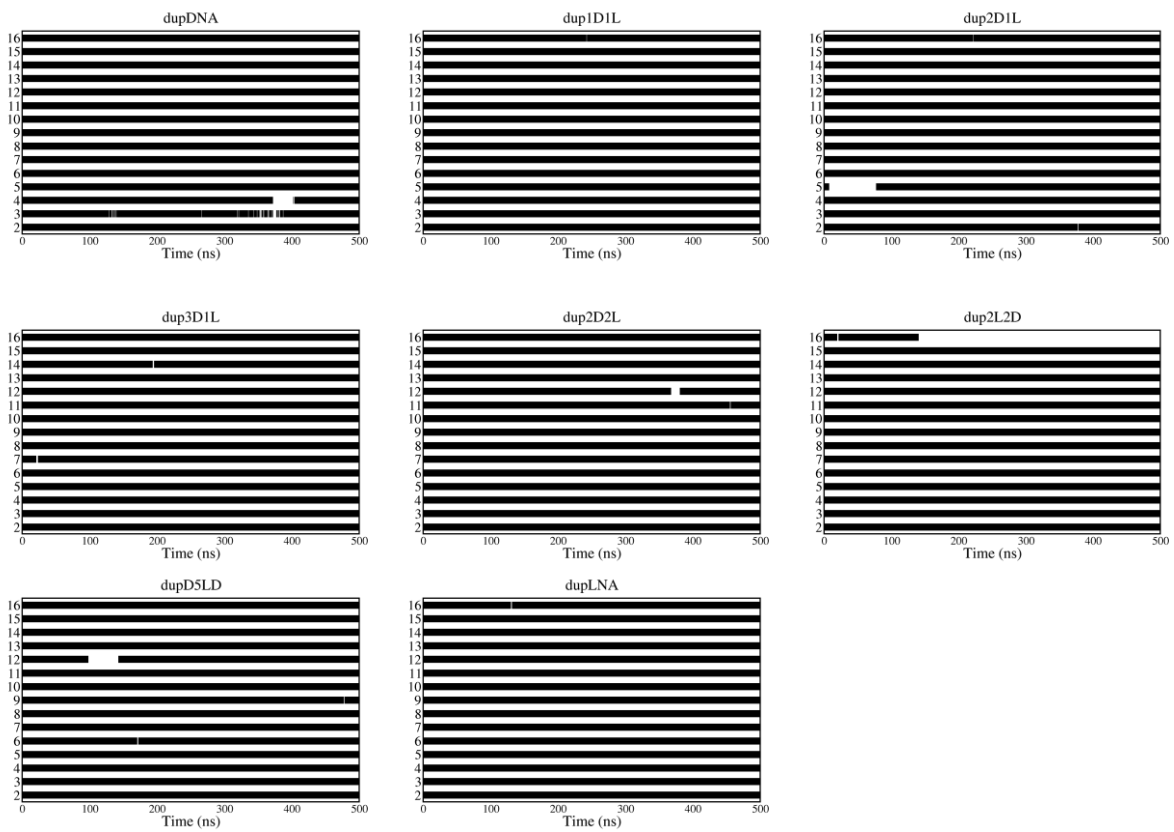
Fig S1. The resistance of base pairs in duplexes as the function of simulation time. The stripes are filled by the snapshots with closed WC base pairs, whereas left blank if the snapshots with opening WC base pairs. The end base pairs (bp.1 & 17) are not shown.
