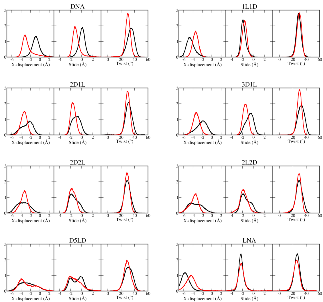
Fig S3. The selected base pair geometries (x-displacement, slide and twist) of each duplex and corresponding triplex. The histograms were sampled from 500 ns simulations. The triplex conformations are shown in red and duplexes are in black.
