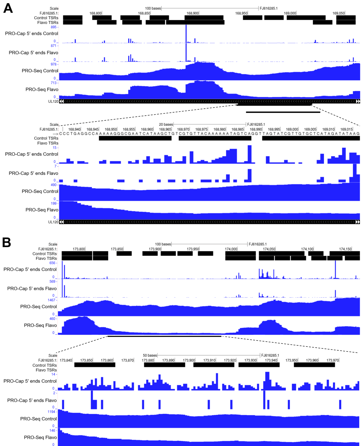
Fig. S1. Comparison of TSRs from the HCMV Towne control and flavopiridol datasets. TSR, PRO-Seq and 5' ends from PRO-Cap tracks are shown (forward direction only).
