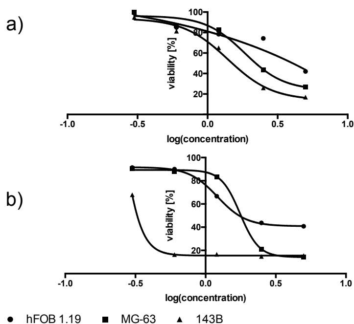
Fig. Log(concentration) vs. cell viability plots. Non-linear regression analysis: log(inhibitor) vs. normalized response has been performed to calculate log IC 50 values. Calculation were made for three cell lines (hFOB1.19, MG-63 and 143B), using (a) MTT and (b) NR assay. The obtained data are reported as the mean ± SD for triplicate determination of 3 separate experiments
