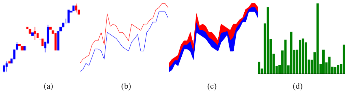
Fig. An example of four stock chart images using SPY data in testing dataset. (a) Candlestick chart, (b) Line chart, (c) F-line chart, and (d) Bar chart
