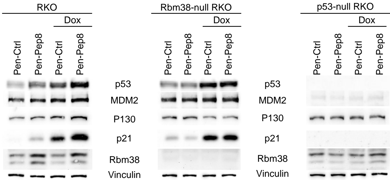
Supplementary Fig. 5. Pep8 sensitizes tumor cells to doxorubicin induced senescence. Immunoblot for wild-type, Rbm38- and p53-null RKO cells treated with Pen-Ctrl or Pen-Pep8 (5 \mu M) with or without 6.25 ng/mL doxorubicin for 18 h.
