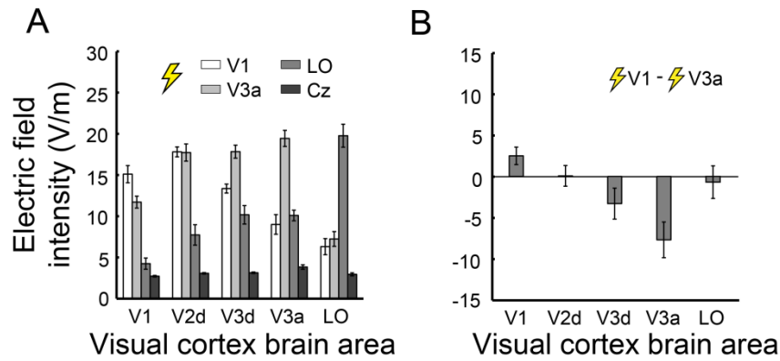
Fig. S2 A) Mean simulated electric field intensity in functional areas of the visual cortex for stimulation over V1, V3a, LO and Cz. Error bars depict one standard deviation. B) Mean contrast of simulated electric field intensity for stimulation over V1 and V3a. Error bars depict one standard deviation. Both stimulation over V1 and V3a produced comparable stimulation over early visual areas outside V1 e.g. V2d, however only V1 stimulation produced significant changes in behavior. This contrast acts as an estimate of behaviorally meaningful stimulation.
