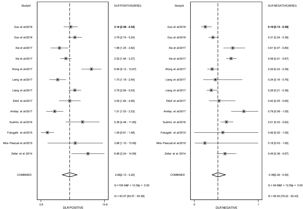
Figure S3: Pooled DLR of fecal Fusobacterium nucleatum for colorectal cancer
