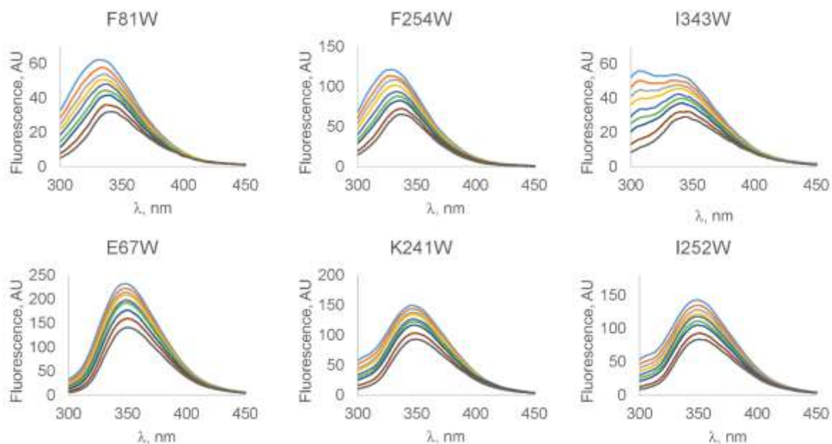
Figure S8. Fluorescence spectra of AcrA single Trp mutants in the presence of increasing concentrations of clorobiocin.
