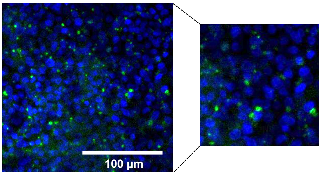
Supplementary Figure 1. Disposition of 5 (and 6)-carboxy-2',7'-dichlorofluorescein (CDF) (green) in 1-week cultures of Huh7 cells. Nuclei were visualized with DAPI (blue). Huh7 cell cultures were treated for 10 min with 2 \mu\text{M} CDF diacetate and 5 \mu\text{M} DAPI, followed by washes with HBSS and confocal microscopy.
