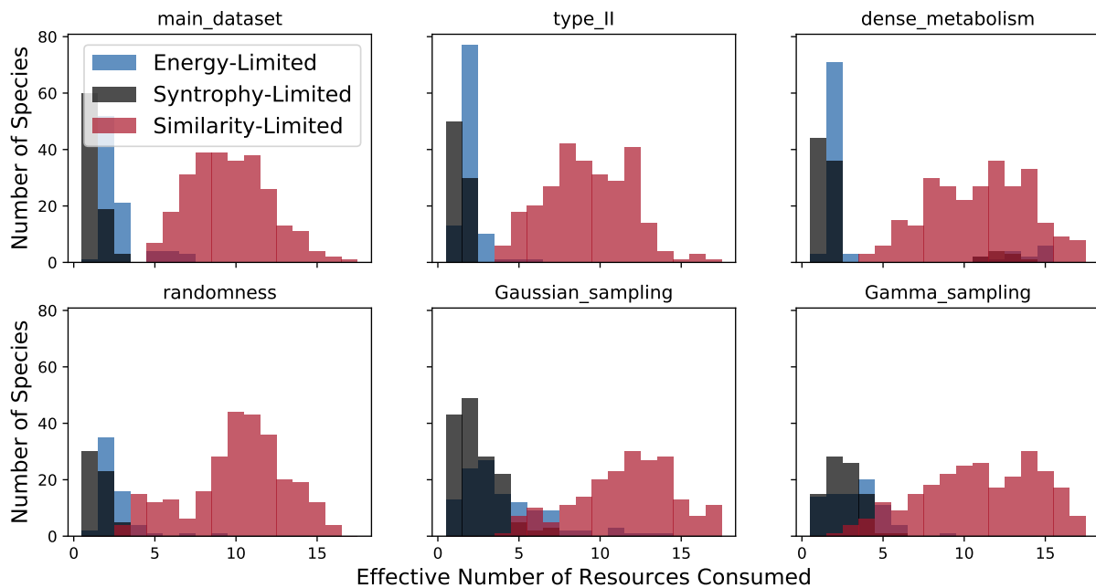
Figure S5: Effective number of resources consumed under different modeling choices. The effective number of resources consumed M_i^{\text{eff}} is computed as described in the main text for the three examples highlighted in Figure 2, for each of the six model choices listed at the beginning of Supporting Text Section 3. The y axis indicates the total number of species falling into each bin from the combination of all 10 parallel communities in each example.
