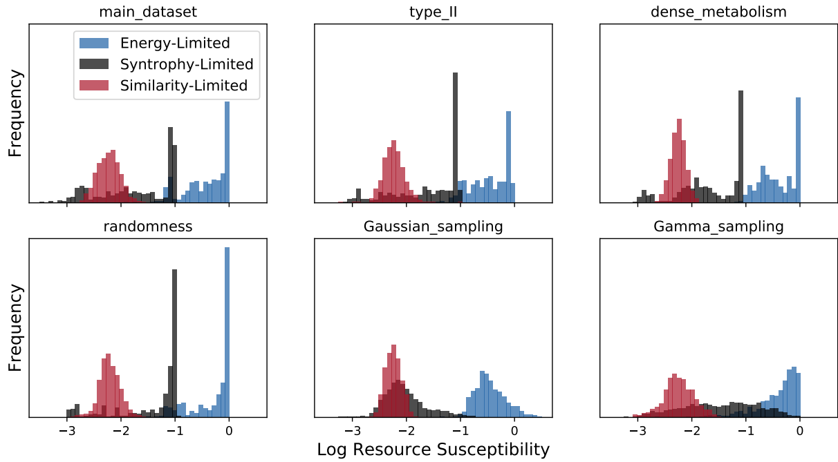
Figure S6: Resource susceptibility. Histograms of the logarithm \log_{10} \partial \bar{R}_\alpha / \partial \kappa_\alpha are plotted for the three examples highlighted in Figure 2, for each of the six model choices listed at the beginning of Supporting Text Section 3. The y axis indicates the total number of species falling into each bin from the combination of all resources for all 10 parallel communities in each example, excepting the externally supplied resource \alpha = 0 .
