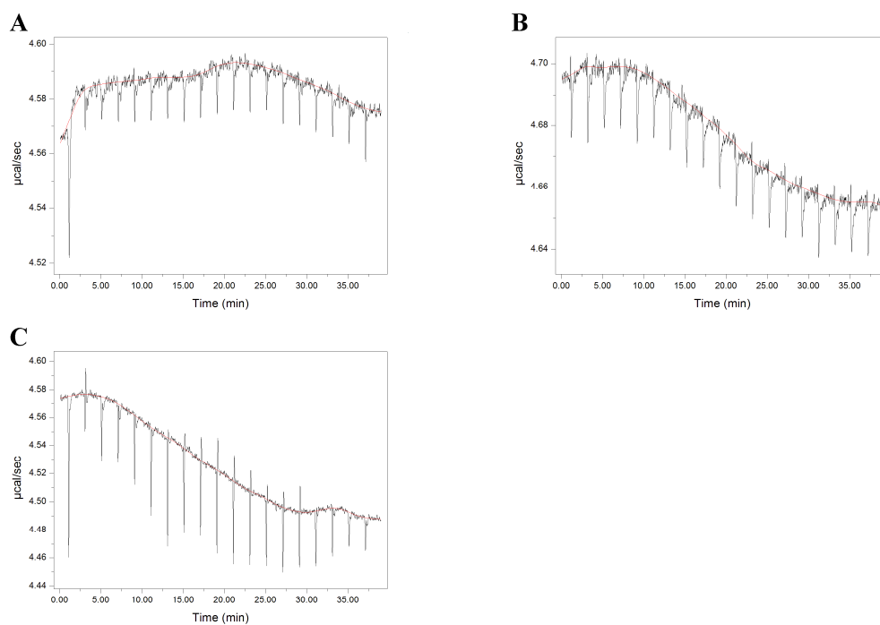
Figure S1. Properties of cations binding to tau-R3. (A) (B) and (C) ITC profiles for the binding of Mn 2+ , Mo 5+ or Fe 3+ to Tau-R3, respectively.
