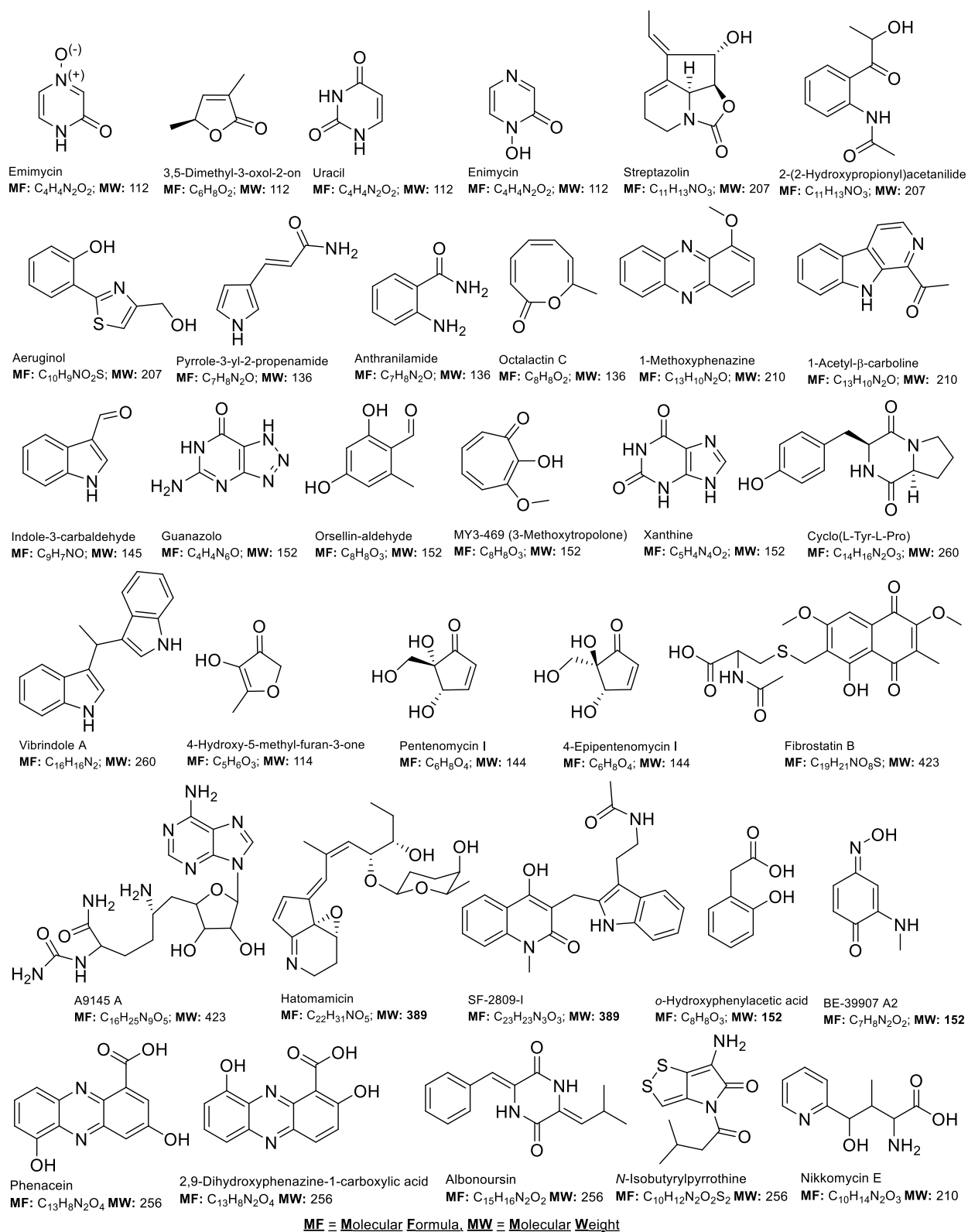
Figure S19: Chemical structures of the suggested Streptomyces metabolites based on HPLC-UV/Vis and LC-MS analyses and by searching in AntiBase 2017.
