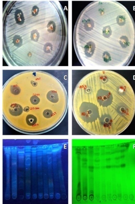
Figure S2: Antibacterial activity of the selected actinobacterial strains against MRSA isolates: (A, B) Zone of inhibition in agar plug method, (C, D) zone of inhibition in well method, (E) different bands of crude extracts of actinomycete isolates under UV at 366nm (F) at 254nm wavelength.
