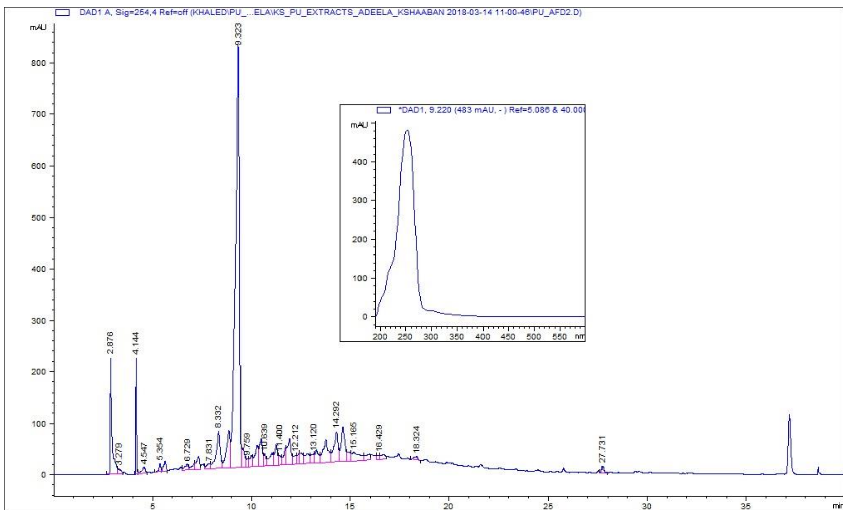
Figure S3. HPLC/UV analyses of AFD2 crude extract. HPLC-conditions: Detection wavelength 254 nm; solvent A: H 2 O/0.1% TFA; solvent B: acetonitrile; flow rate: 1.0 mL min -1 ; 0-30 min, 95-0% A (linear gradient); 30-35 min 0% A; 35-36 min 0-95% A (linear gradient); 36-40 min 95% A.
