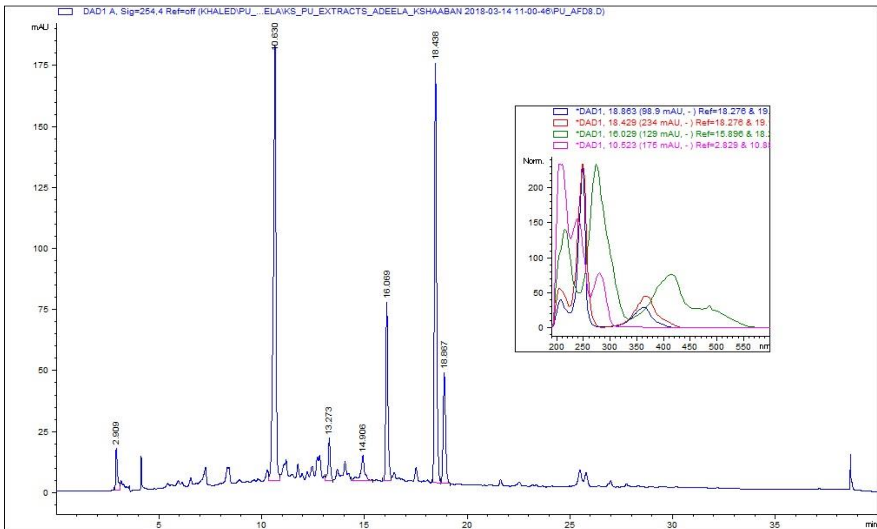
Figure S9. HPLC/UV analyses of AFD8 crude extract. HPLC-conditions: Detection wavelength 254 nm; solvent A: H 2 O/0.1% TFA; solvent B: acetonitrile; flow rate: 1.0 mL min -1 ; 0-30 min, 95-0% A (linear gradient); 30-35 min 0% A; 35-36 min 0-95% A (linear gradient); 36-40 min 95% A.
