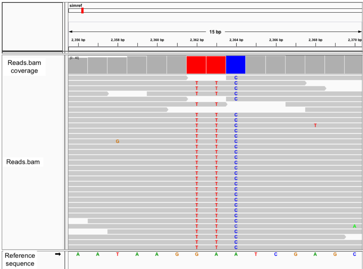
Figure 1: SNPs in IGV viewer. This figure illustrates a view of a section of mapped reads in the dataset simulated by HMM. It shows three SNPs at base 2362 (G → T), 2363 (A → T) and 2364G (A → C).
