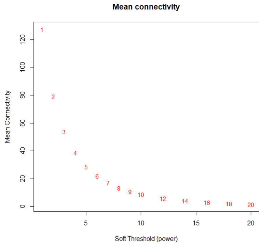
Supplementary Figure 1. Picking up a soft-threshold approximating to a scale free topology criterion based on R square and mean connectivity
