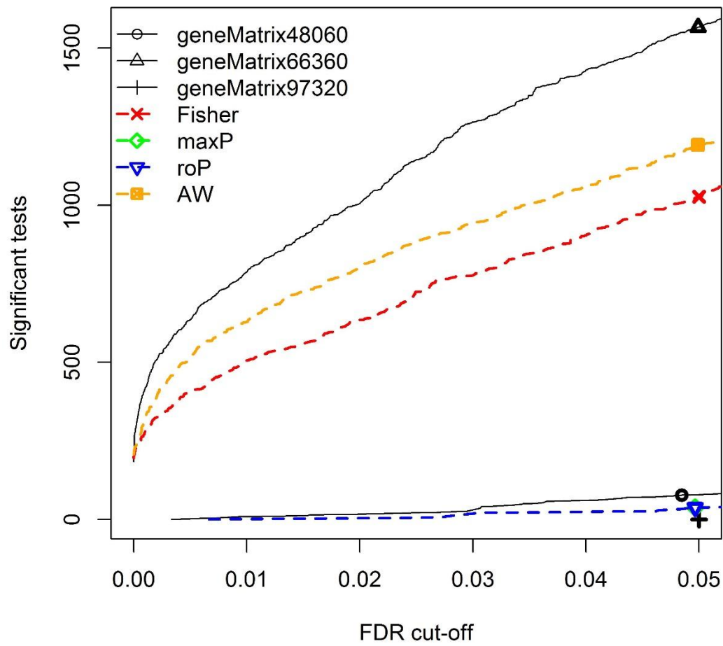
Supplementary Figure 2. Number of detected DEGs under different q -value threshold
