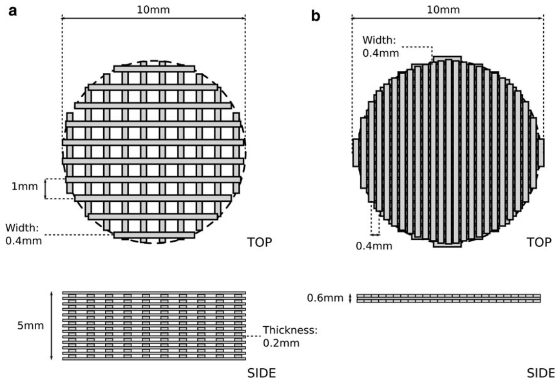
SUPPLEMENTARY FIG. S1. Annotated schematic of the 3D-printed PCL/ \beta -TCP (80:20) scaffolds used in the experiments: (a) scaffold used for physical properties assessment, (b) scaffold used for biological evaluation.
