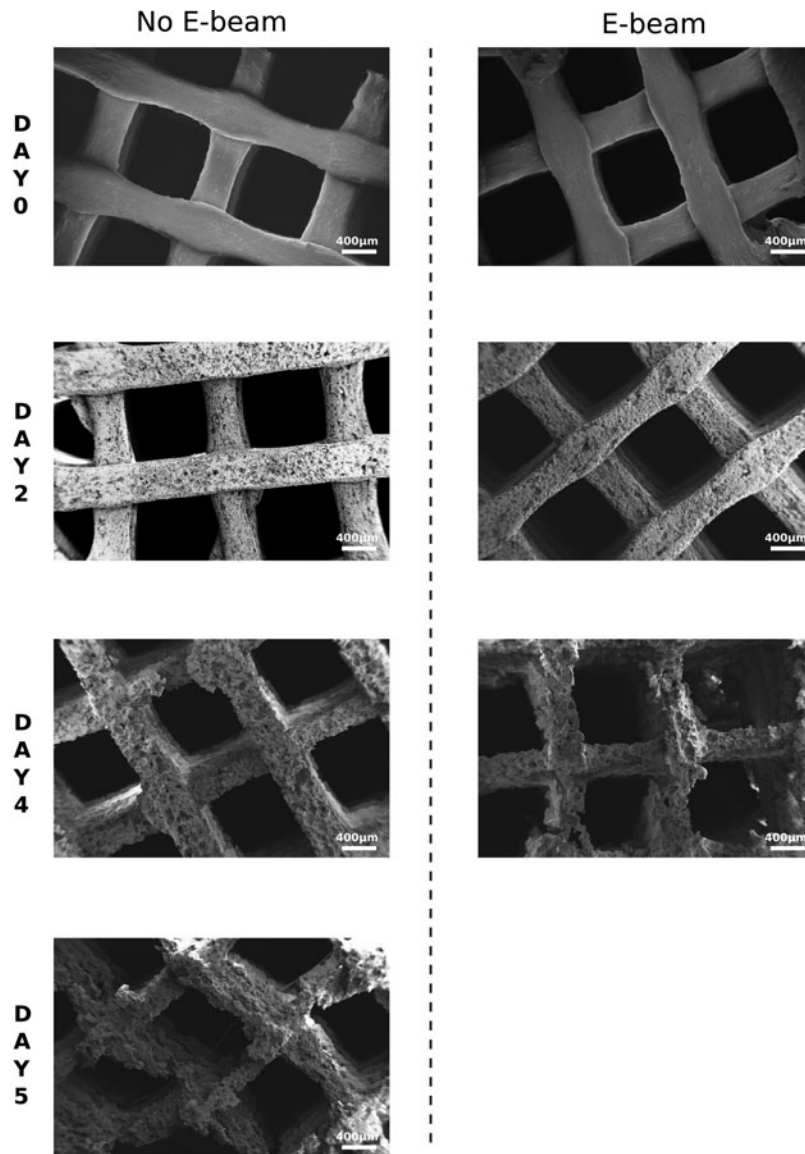
SUPPLEMENTARY FIG. S3. SEM images of 3D-printed PCL/ \beta -TCP (80:20) scaffolds during degradation under alkaline conditions, at days 0, 2, 4, and 5. Two groups are compared: exposed and not exposed to E-beam sterilization. Two magnifications are presented: \times 90 (first page) and \times 5000 (second page).
