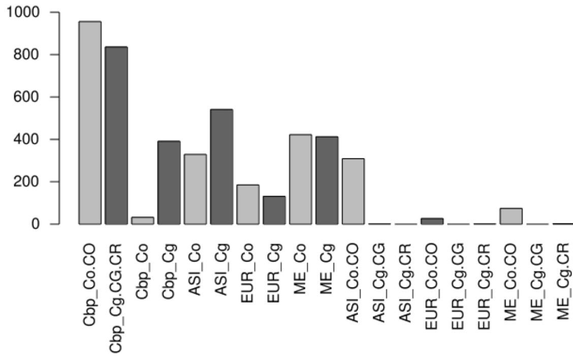
S2 Figure. Frequency of monophyly of different groups. ASI, EUR and ME are the three populations of C. bursa-pastoris (Cbp) with Co and Cg indicating two subgenomes. CO, CG, CR are short forms for C. orientalis , C. grandiflora , and C. rubella respectively.
