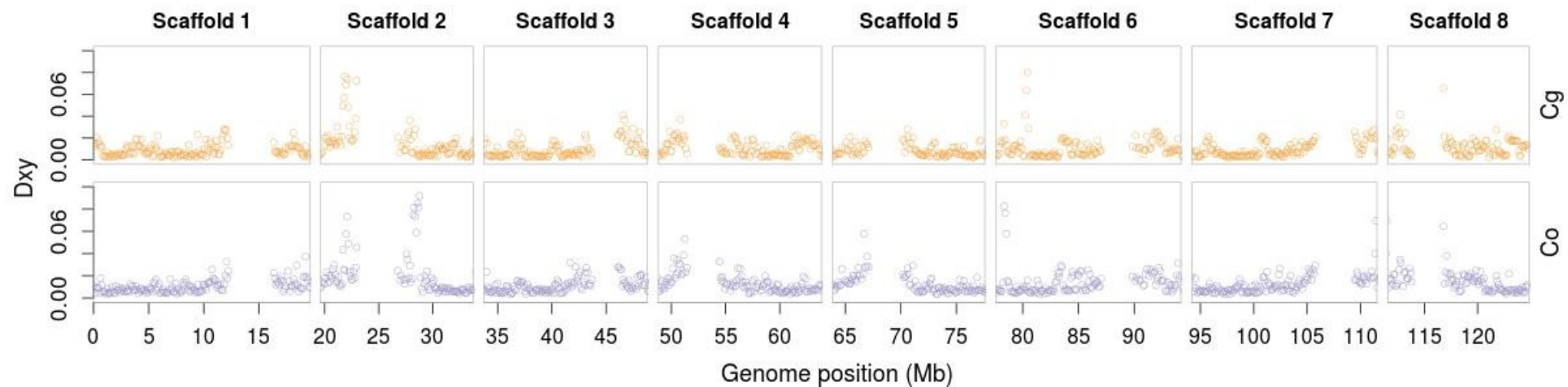
S8 Figure. Genetic distance ( D_{xy} ) between the data analyzed in this study and the assembly of C. bursa-pastoris by Kasianov et al. (2017). The corresponding subgenomes are marked with Cg and Co. Estimates were assessed for 100K windows on SNPs data and scaled to whole genome values.
