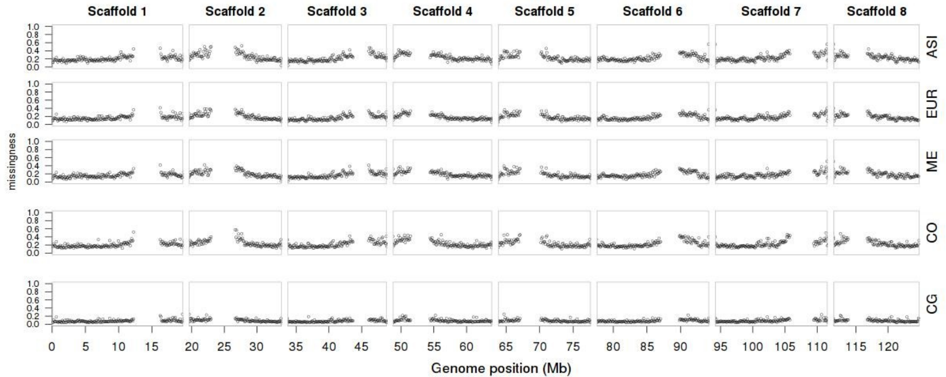
S21 Figure. Variation in the proportion of missing data in populations of C. bursa-pastoris and diploid species. All values have been estimated with sliding windows of 100K genomic positions on the final dataset that was used in the analyses. ASI, EUR and ME are the three populations of C. bursa-pastoris . CO and CG are short forms for C. orientalis and C. grandiflora , respectively. The regions without the data mostly correspond to pericentromeric regions that were excluded from the data.
