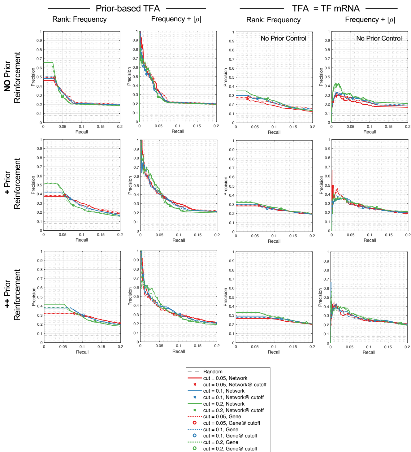
Figure S27. StARS parameterization: precision-recall of the KO+ChIP G.S. TRNs were built using the Th17 ATAC prior with prior-based or TF mRNA TFA, no, moderate or strong prior reinforcement, network- and gene-level average instabilities at cutoffs .05, .1 and .2. Edges are ranked according to nonzero subsamples or Equation 4 .
