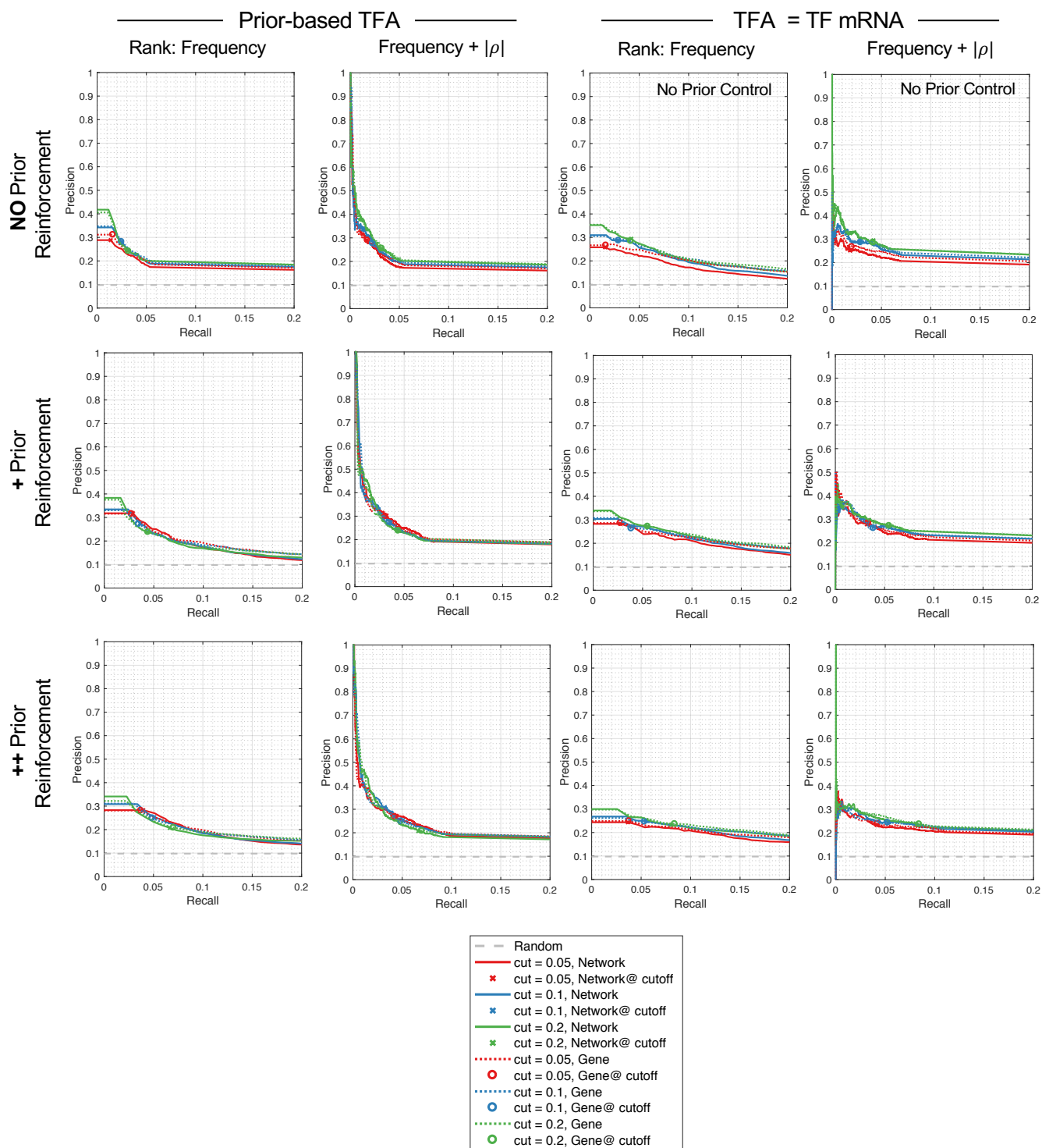
Figure S28. StARS parameterization: precision-recall of the KO G.S. TRNs were built using the Th17 ATAC prior with prior-based or TF mRNA TFA, no, moderate or strong prior reinforcement, network- and gene-level average instabilities at cutoffs .05, .1 and .2. Edges are ranked according to nonzero subsamples or Equation 4 .
