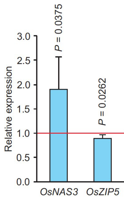
S1 Fig. Expression change of OsNAS3 (Os07g0689600) and OsZIP5 (Os05g0472700) under elevated [CO 2 ] condition relative to ambient [CO 2 ]. Actin ( Act1 ) was used as the control. Data are presented as mean \pm s.d. (n = 3). Student's t-tests were used to calculate P values.
