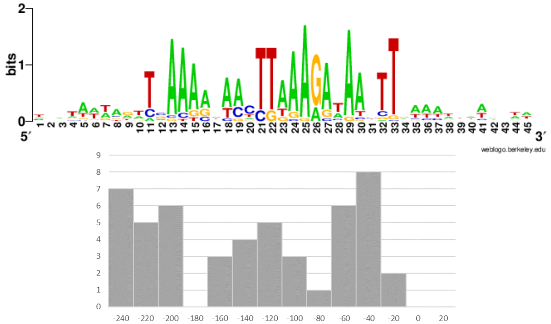
Motif #7 (50 sites)
