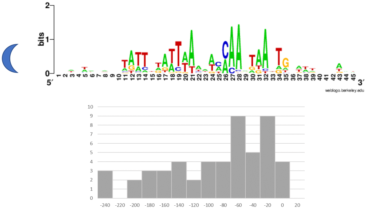
Motif #4 (62 sites)
