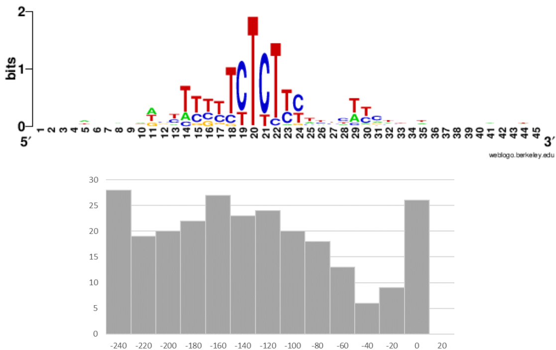
Motif #7 (255 sites)
