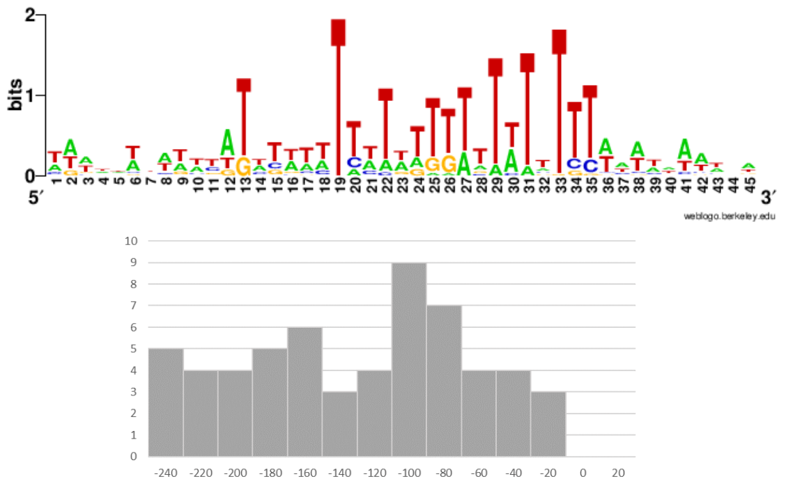
Motif #7 (58 sites)
