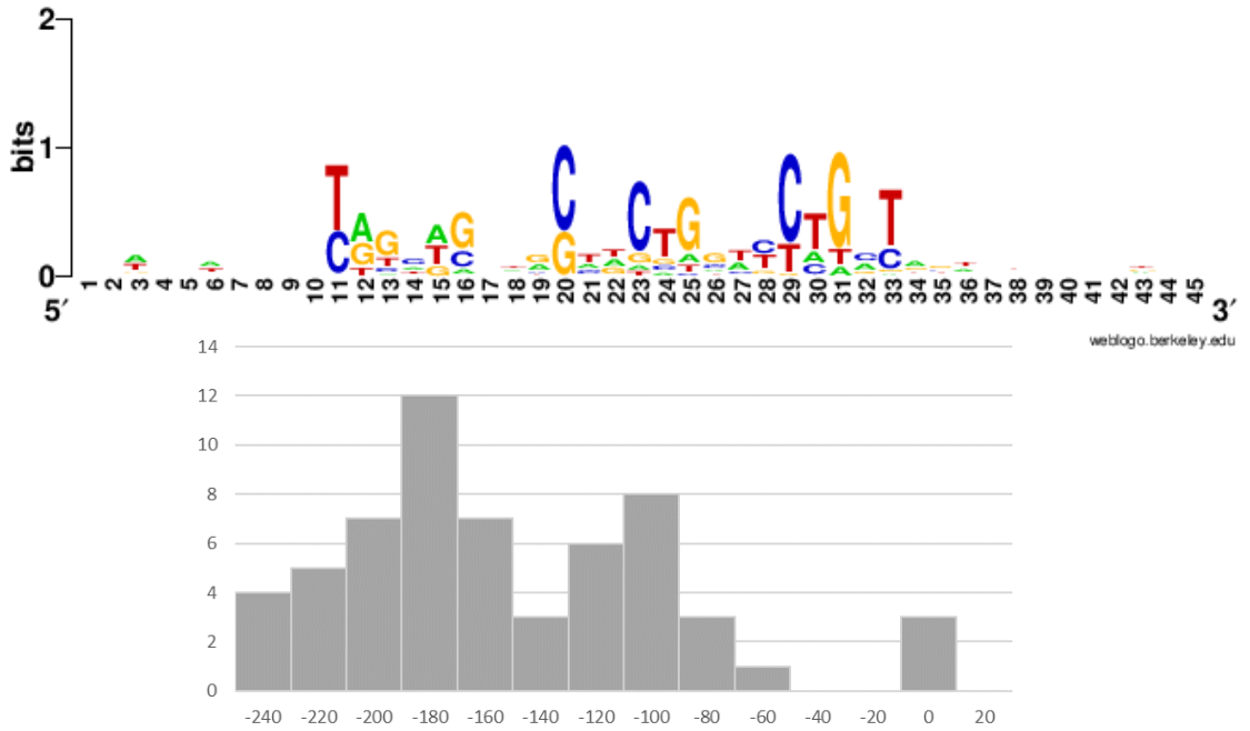
Motif #3 (59 sites)
