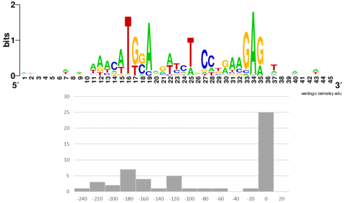
Motif #7 (52 sites)
