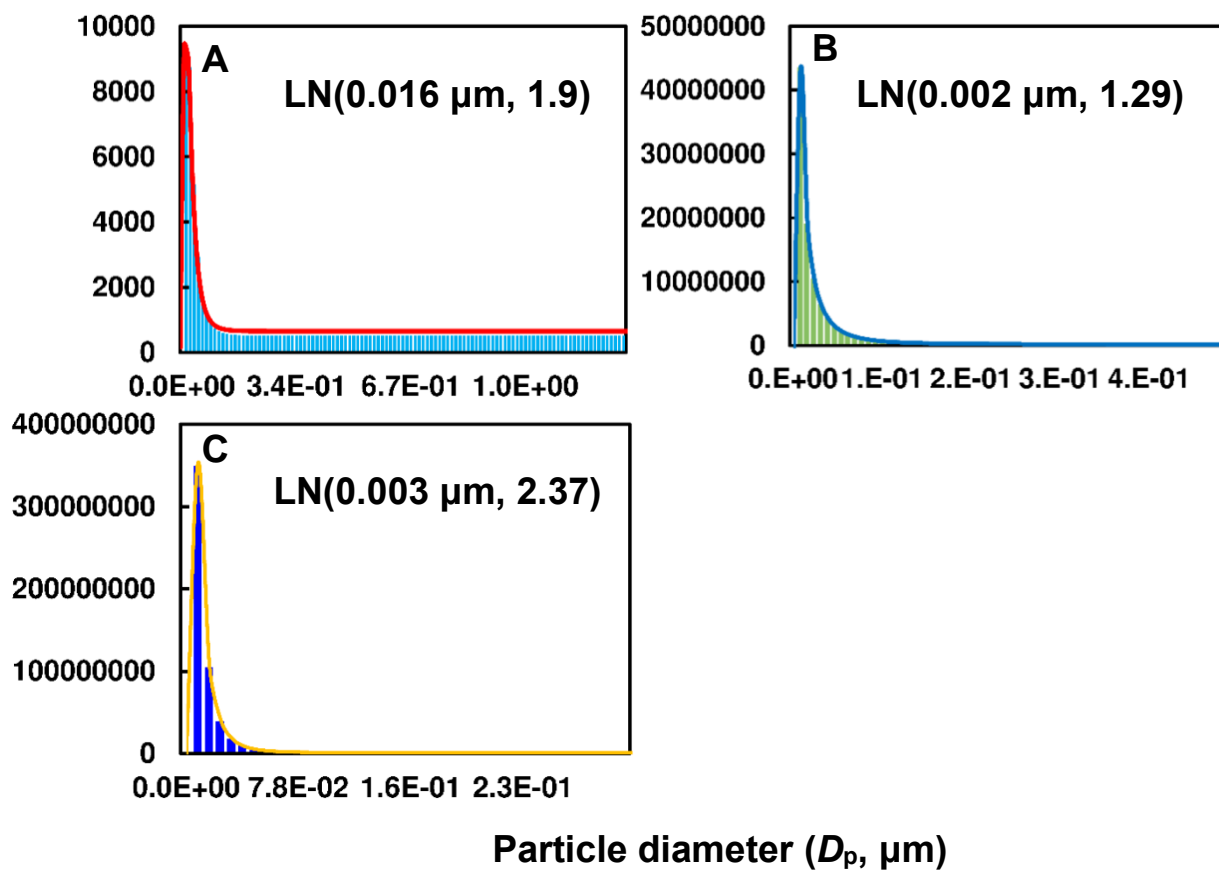
Fig. S1. Estimated size distributions (in the unit of size-dependent number concentration) of droplets in spray (A) DI, (B) DO S , and (C) DO L .
