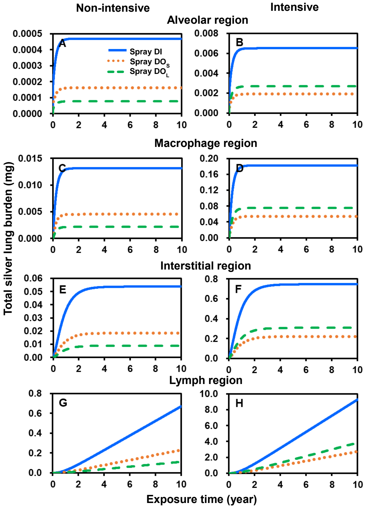
Fig. S2. Time-dependent silver depositions in regions of (A, B) alveolar, (C, D) macrophage, (E, F) interstitial, and (G, H) lymph nodes when exposed to three kinds of AgNPs-containing spray products in non-intensive or intensive application.
