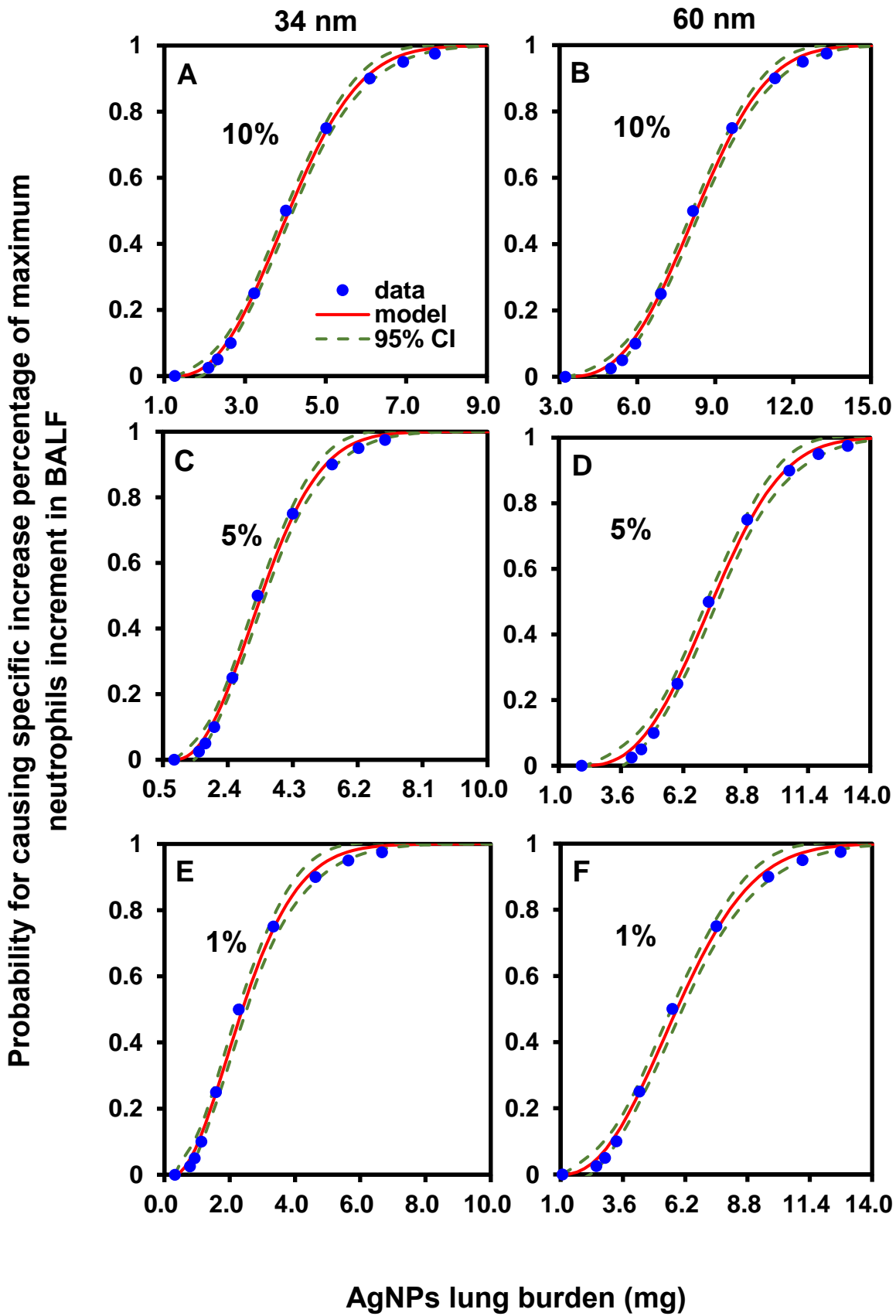
Fig. S3. Best fit of the Weibull threshold model to the cumulative distribution functions of 10, 5, and 1% maximum neutrophils increment in BALF of male Fischer rats posed by various concentrations of (A, C, E) 34 nm and (B, D, F) 60 nm AgNPs.
