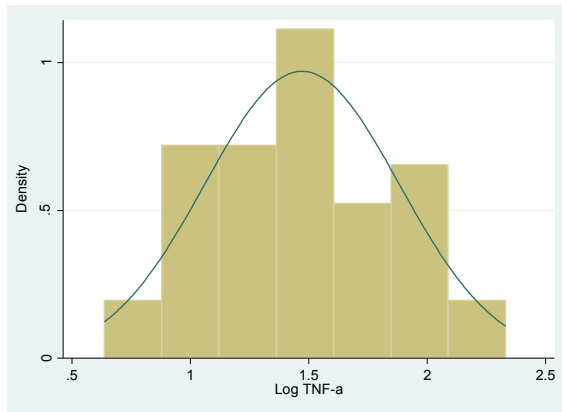
Figure S2. Distributions of log-transformed human variables
