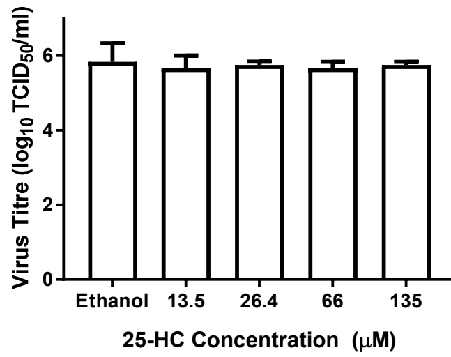
Figure S1. The effect of 25-HC on the viral capsid. Unpurified stocks of MNV were incubated with 25-HC at a range of concentrations or ethanol-only control at 4 h at 37 °C before dilution and measurement of infectivity by TCID 50 assay (n=2 ± SEM).
