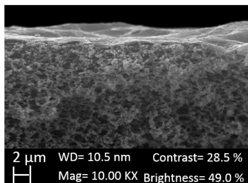
Figure S2. SEM magnification cross-sections of M4, M2 and M5 membranes
