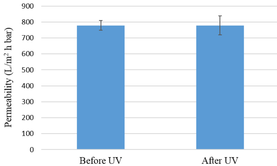
Figure S4. PWP of M8 membrane before and after UV irradiation
