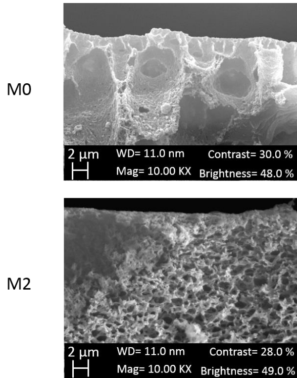
Figure S3. SEM magnification cross-sections of M0 and M2 and M5 membranes
