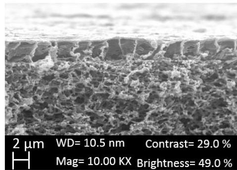
Figure S1. SEM magnification cross-sections of M1, M2 and M3 membranes
