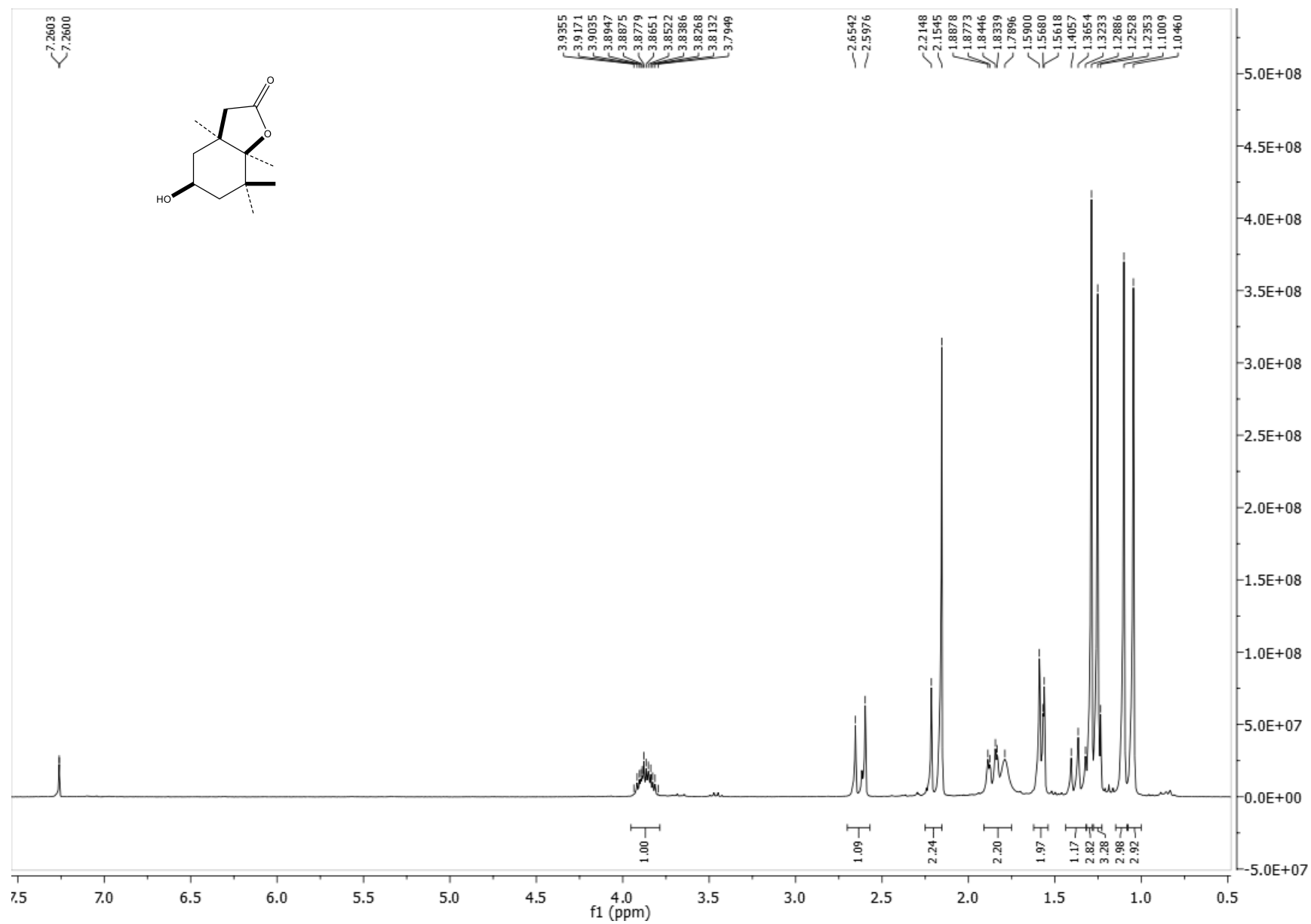
Figure S5. 1 H NMR lactone 3
