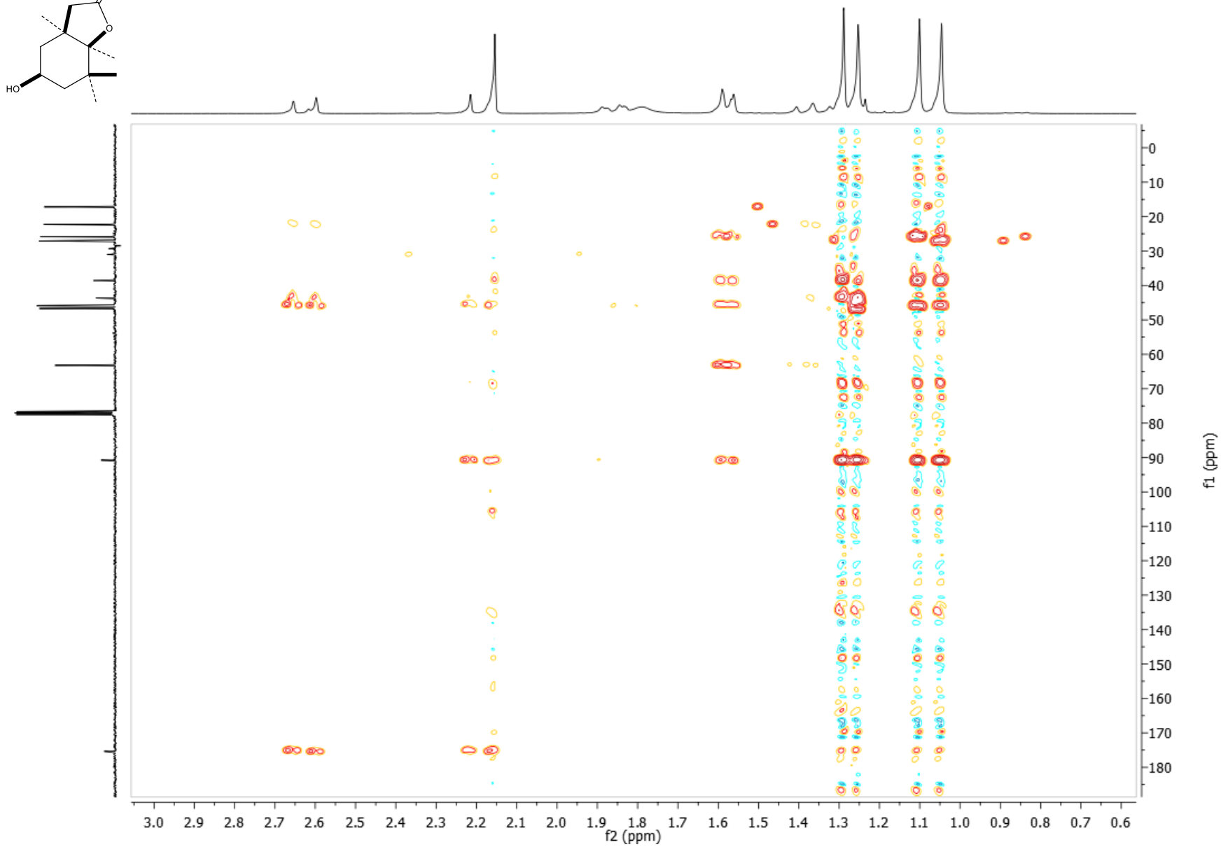
Figure S8. HMBC lactone 3
