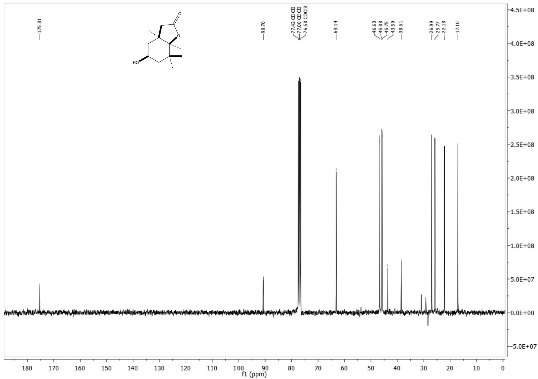
Figure S6. 13 C NMR lactone 3
