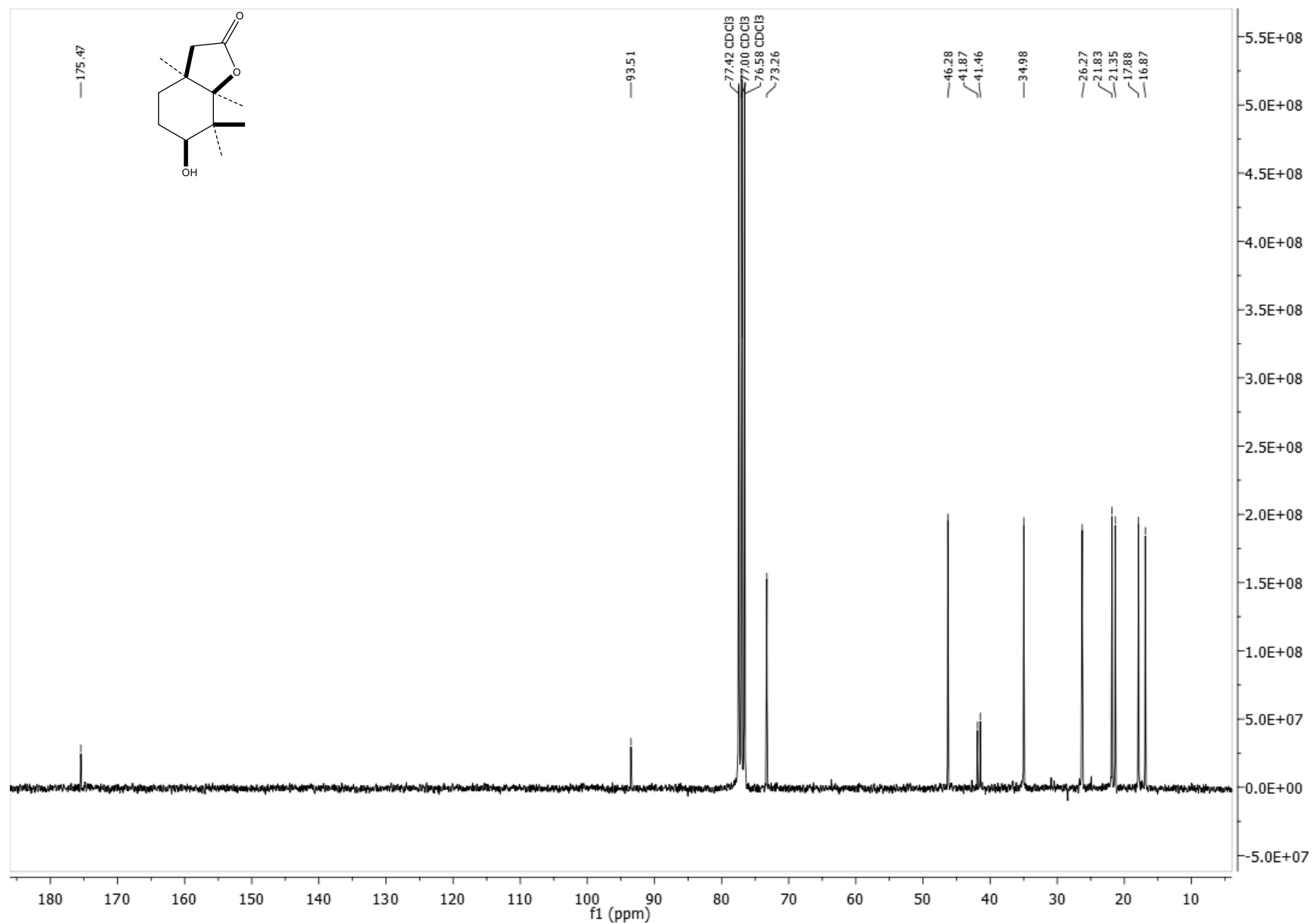
Figure S2. ^{13}\text{C} NMR lactone 2
