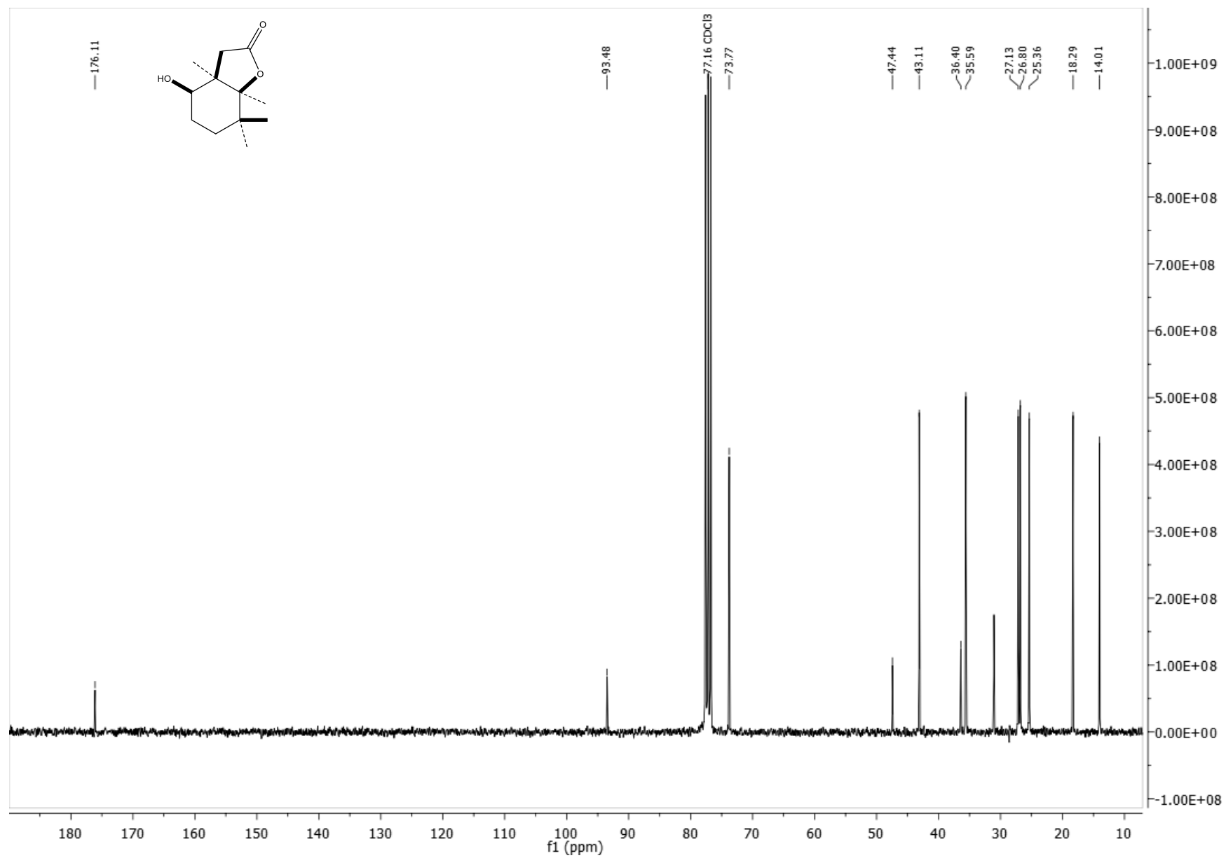
Figure S10. ^{13}\text{C} NMR lactone 4
