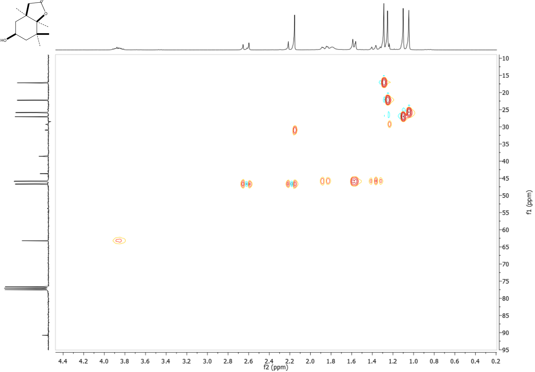
Figure S7. HMQC lactone 3
