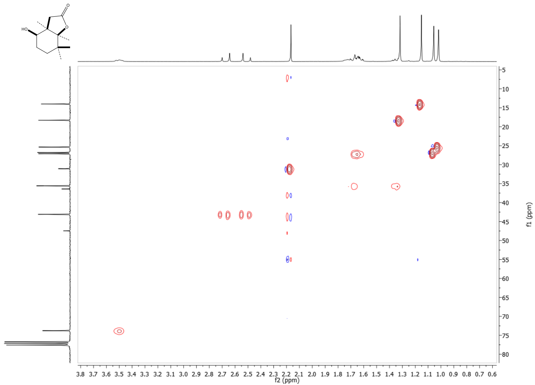
Figure S11. HMQC lactone 4
