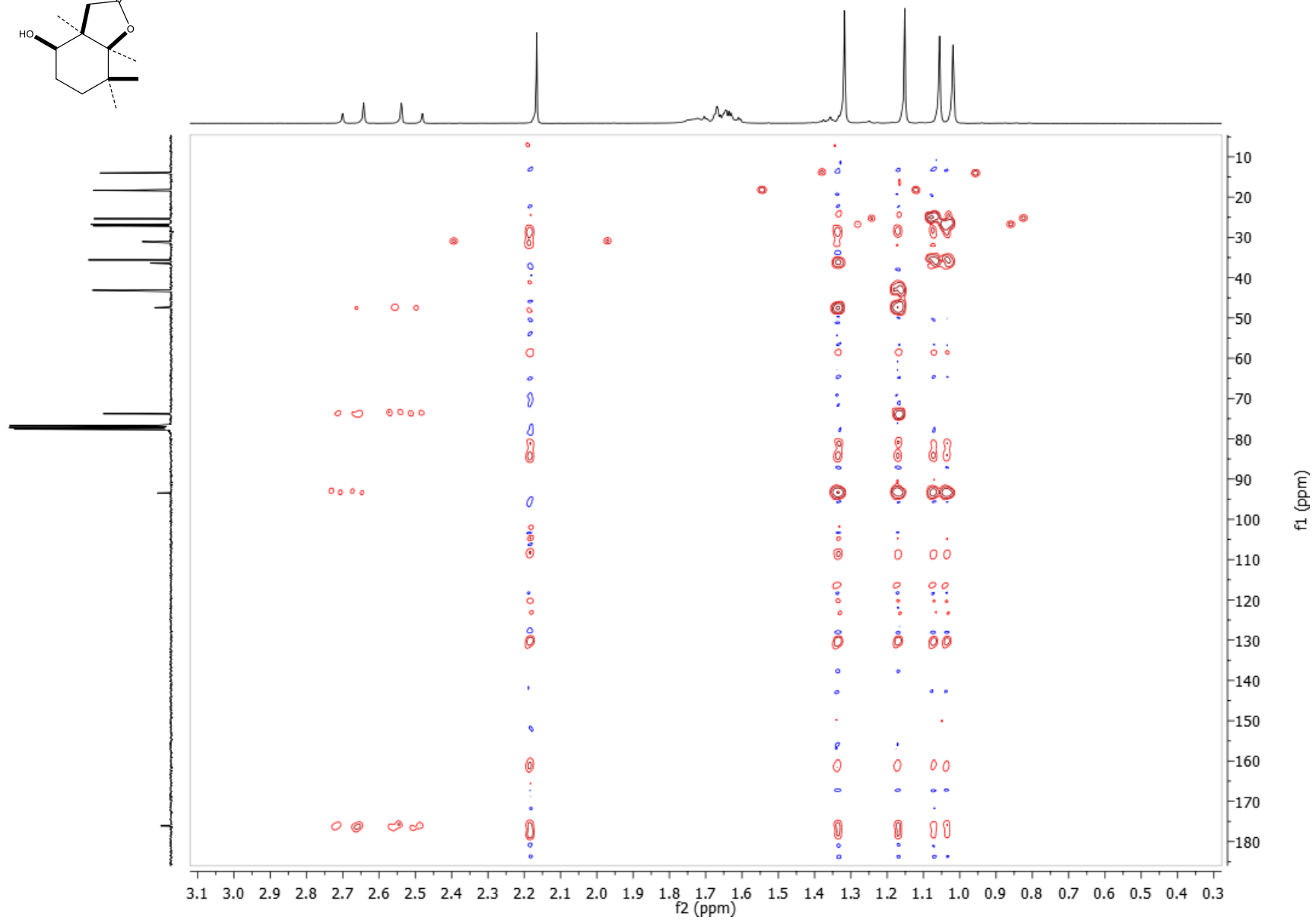
Figure S12. HMBC NMR lactone 4
