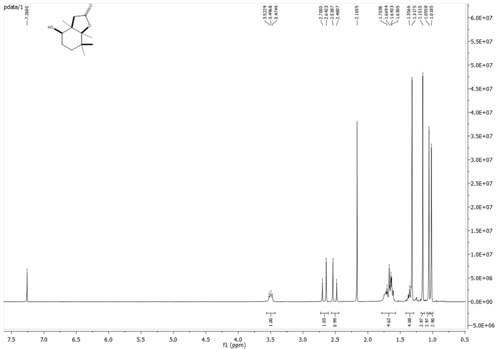
Figure S9. 1 H NMR lactone 4
