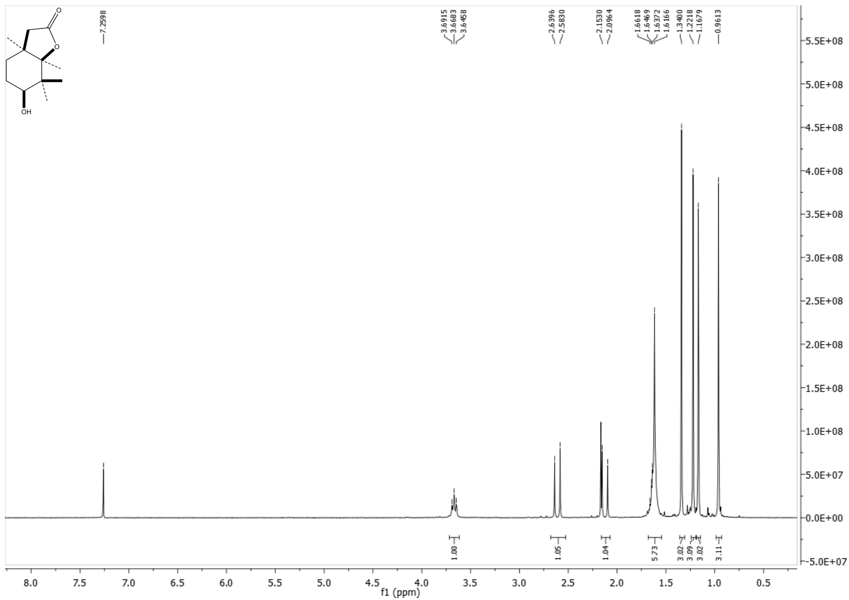
Figure S1. ^1\text{H} NMR lactone 2
