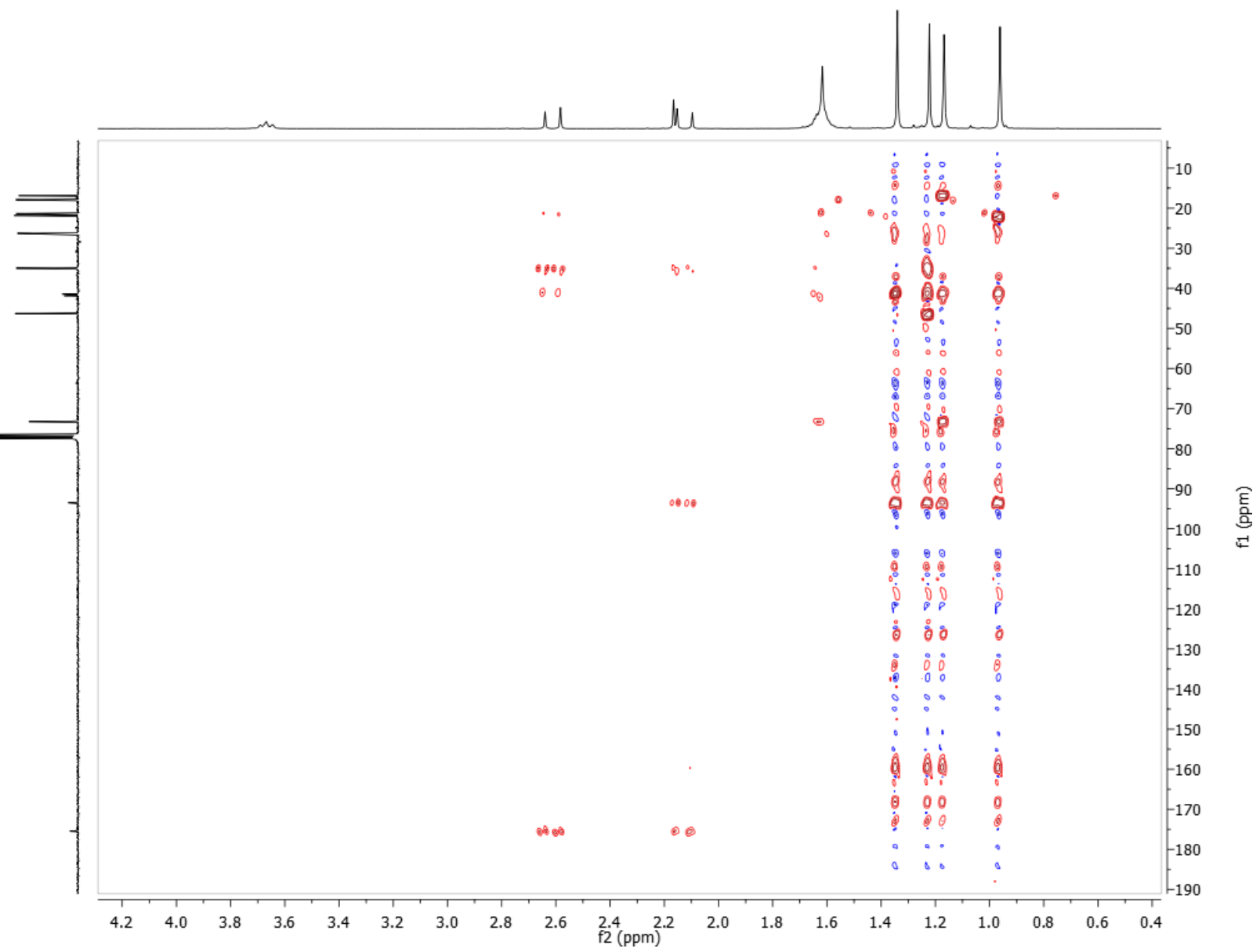
Figure S4. HMBC lactone 2
