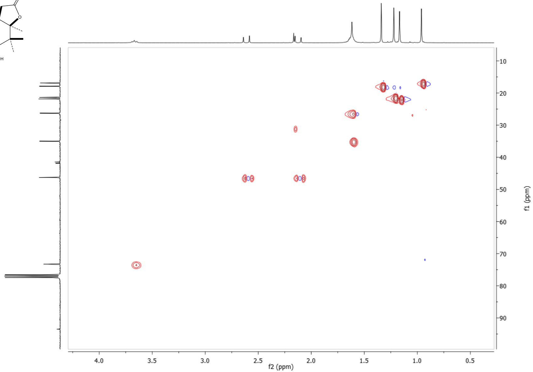
Figure S3. HMBC lactone 2
