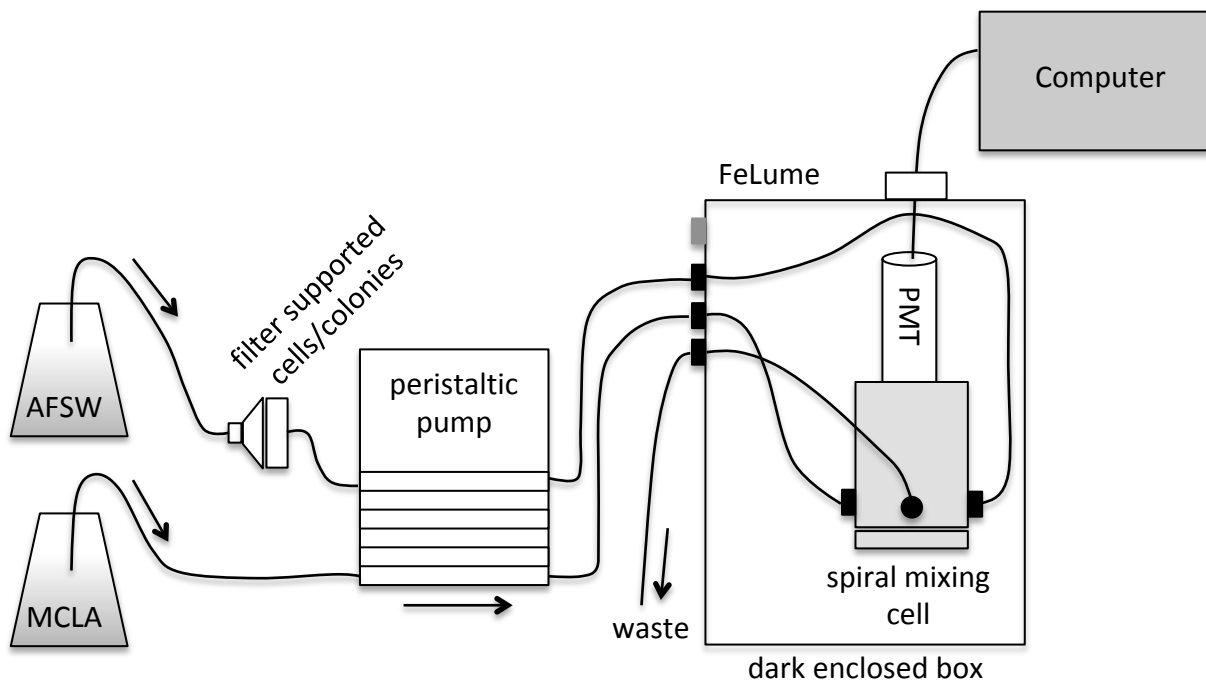
Figure S2. Simplified schematic of the flow injection chemiluminescent approach used to measure extracellular superoxide in this research.
