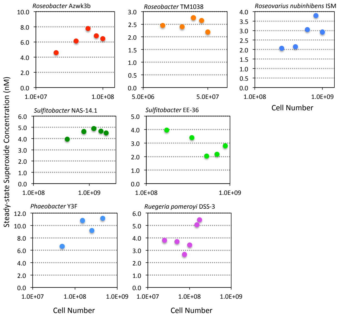
Figure S3. Typical steady-state superoxide concentration trends as a function of cell in mid-exponential cultures of 7 Roseobacter clade species. Here we illustrate the results of one loading experiment as an example of the range of trends observed.
