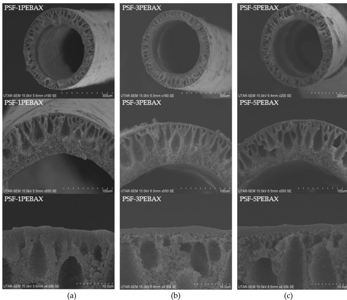
Figure S2. Cross sectional SEM image of PSF membrane coated with PEBAX at concentration of (a) 1 wt %, (b) 3 wt % and (c) 5 wt %.
