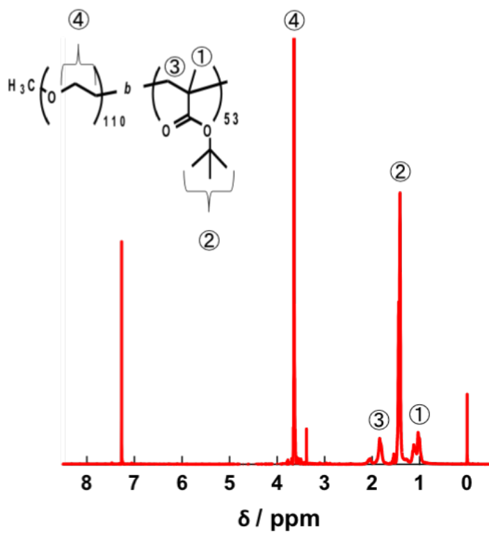
Figure S2. ^1\text{H-NMR} spectrum of PEG- b -PtBMA in \text{CDCl}_3 .
