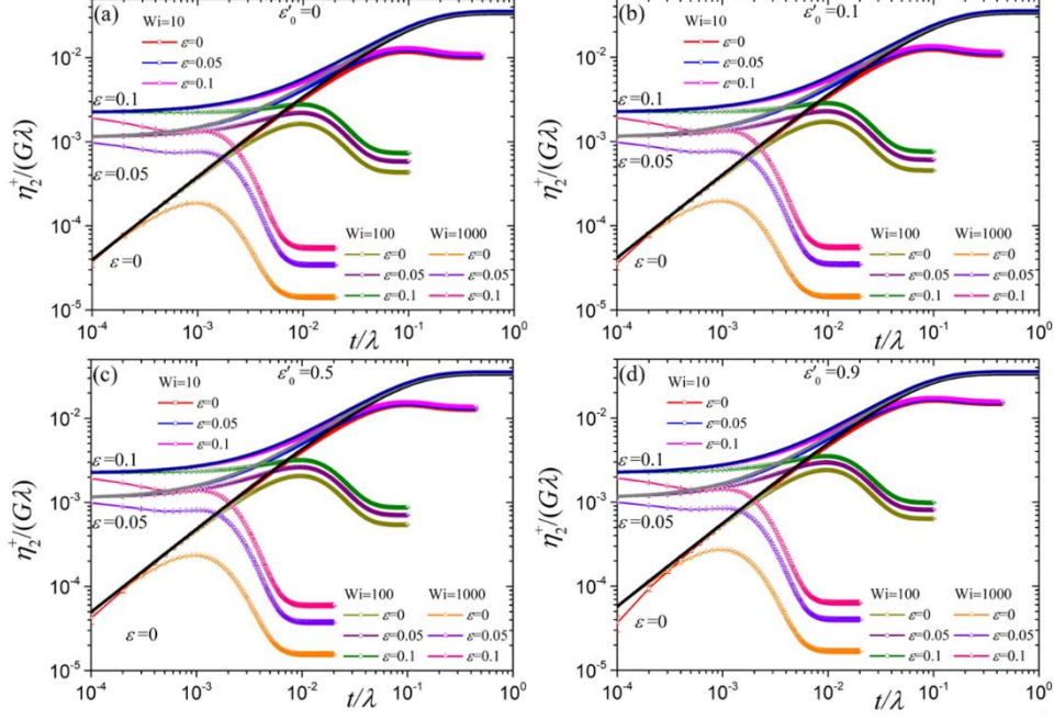
FIG. S4: Same as FIG. S3 but for \eta_2^+ / G\lambda .
