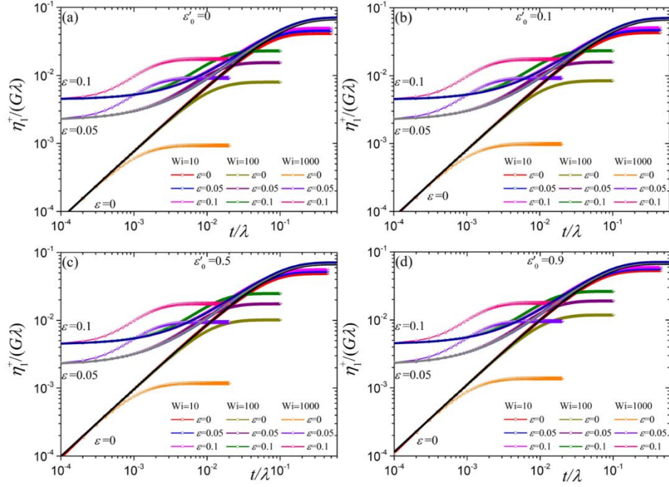
FIG. S3: Predictions for the transient \eta_1^+/G\lambda as a function of time for N=100 and various values of the parameter \varepsilon and dimensionless elongation rate Wi for (a) \varepsilon_0'=0 , (b) \varepsilon_0'=0.1 , (c) \varepsilon_0'=0.5 , and (d) \varepsilon_0'=0.9 . The thick lines give the predictions of Eq. (14).
