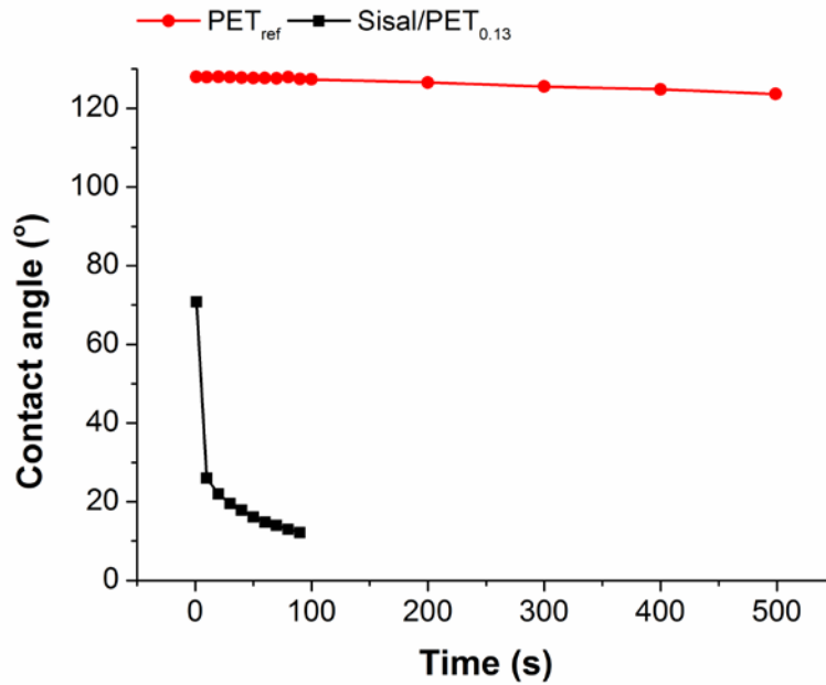
Figure S3: Contact angle curves of PET ref and Sisal/PET 0.13 .
