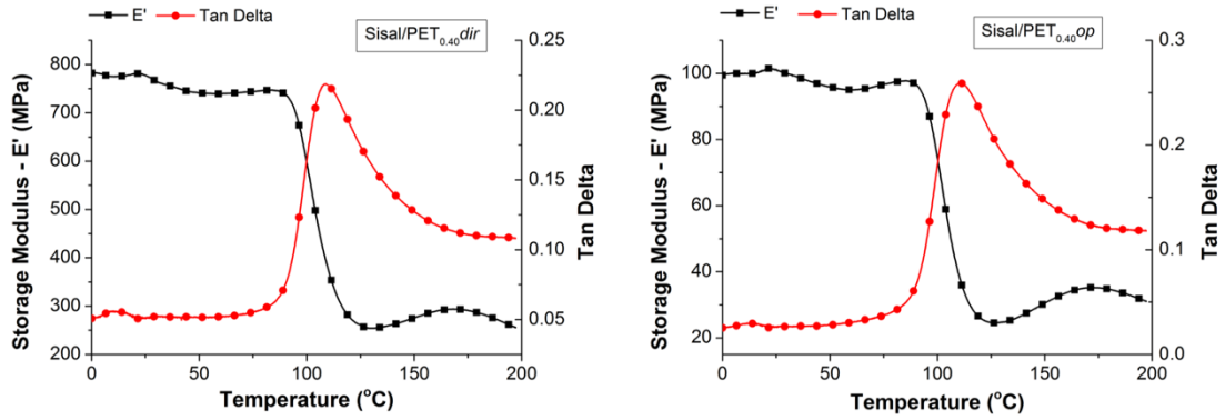
Figure S1: DMA curves of Sisal/PET 0.40 ( dir and op )
