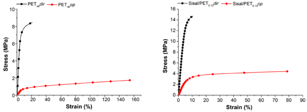
Figure S2: Tensile strength curves of PET ref and Sisal/PET 0.40 ( dir and op )
