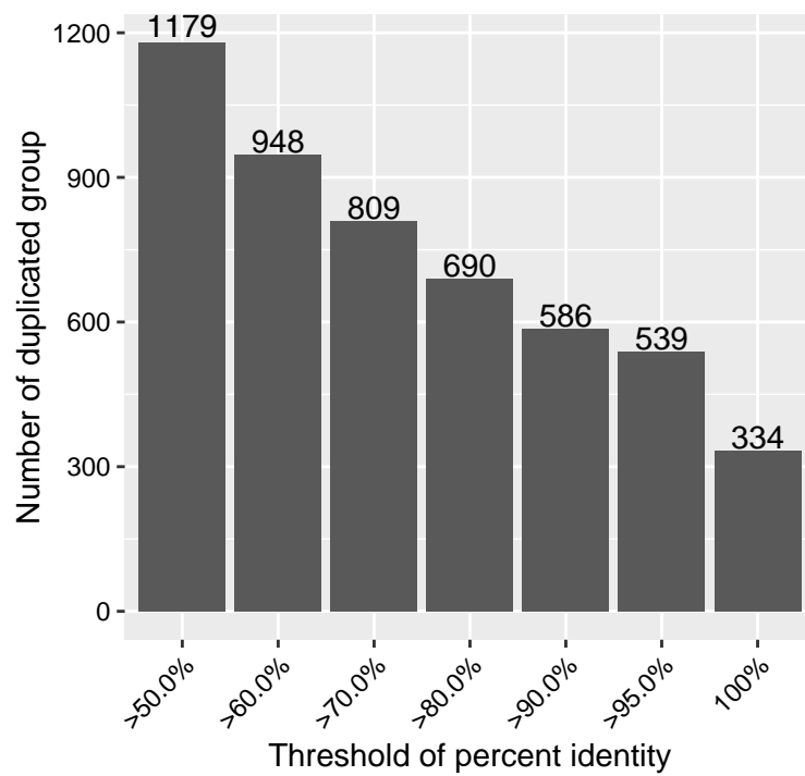
S1 Fig. Number of duplicated genes in the M. marinum S8 genome.
