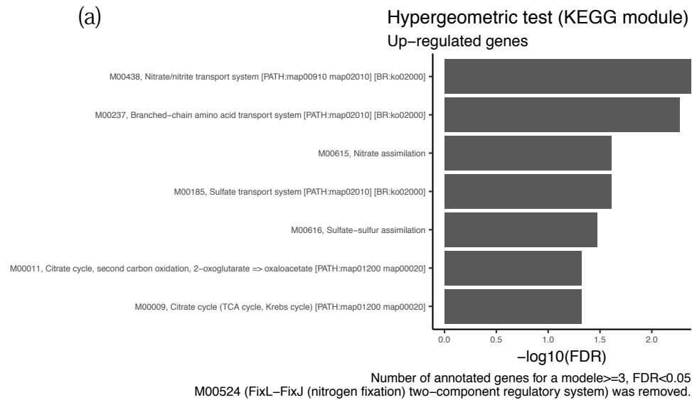
S4 Fig. The results of hypergeometric test for overlaps of KEGG modules with (a) up- or (b) downregulated genes. The modules with \text{FDR} < 0.05 and \geq 3 annotated M. caenitepidi Gela4 genes are shown according to the value of \log_{10}(\text{FDR}) .
