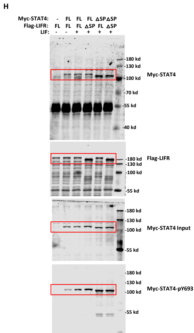
Figure 4. LIF-activated STAT4 is phosphorylated on SPXX motifs within the C-terminal transcription regulation domain.
