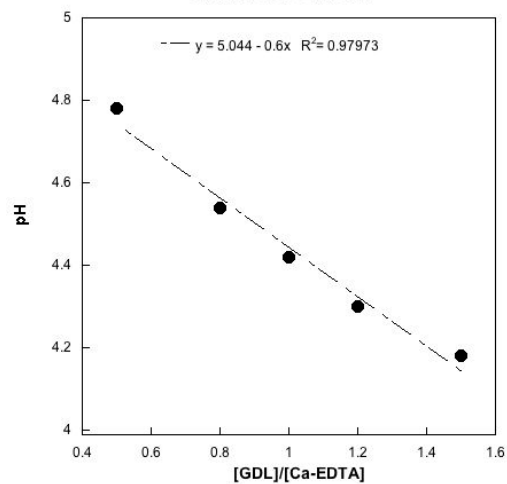
Figure S1. Calibration curve for the pH variation as function of GDL and Ca-EDTA complex.
