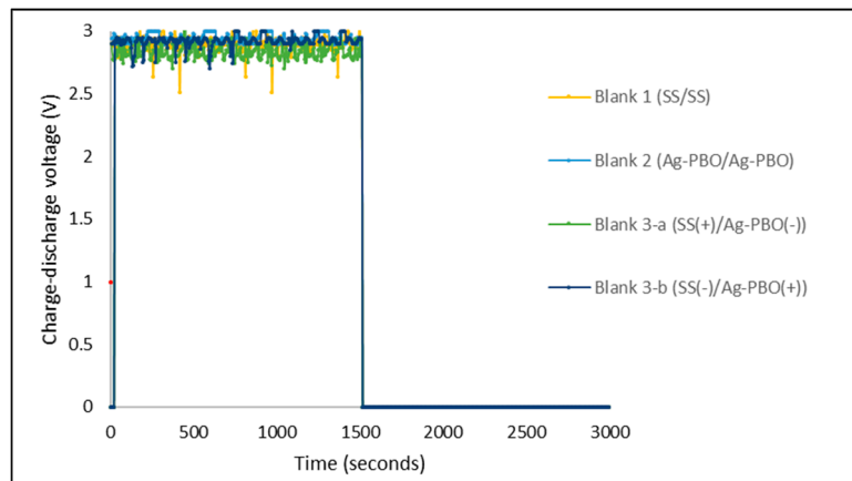
Supplementary Figure 2: Charge-discharge characteristics of blank devices (without PEDOT:PSS) using various electrodes (SS/SS, Ag-PBO/Ag-PBO, SS(+)/Ag-PBO(-), and SS(-)/Ag-PBO(+)), each charged at 3 volt.
