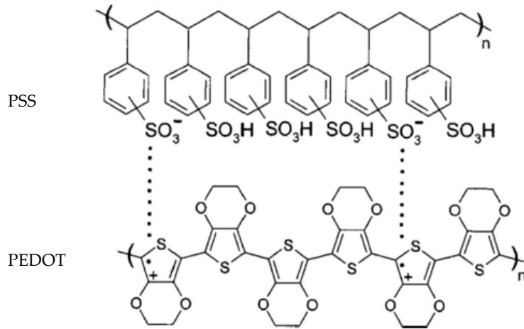
Supplementary Figure 1: Chemical structure of PEDOT:PSS [19]
