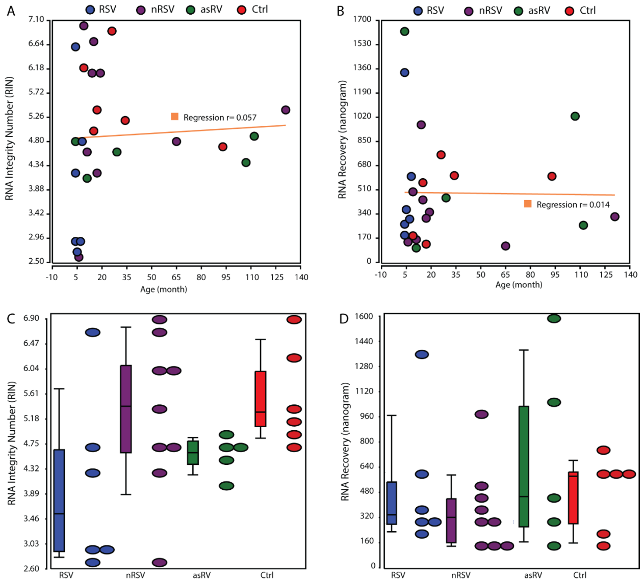
Figure S1. Relationships between RNA quality and quantity with age and study group. Panel A, RIN vs. age; Panel B, RNA recovery vs. age; Panel C, RIN vs. study group; panel D, RNA recovery vs. study group.
